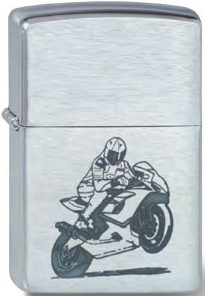
Motorcycle Wheelie 1.100.127 #200 · 39,95 €
