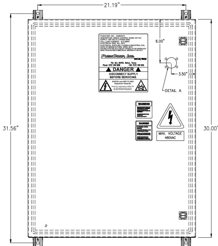
Figure 1. Cabinet Mounting
