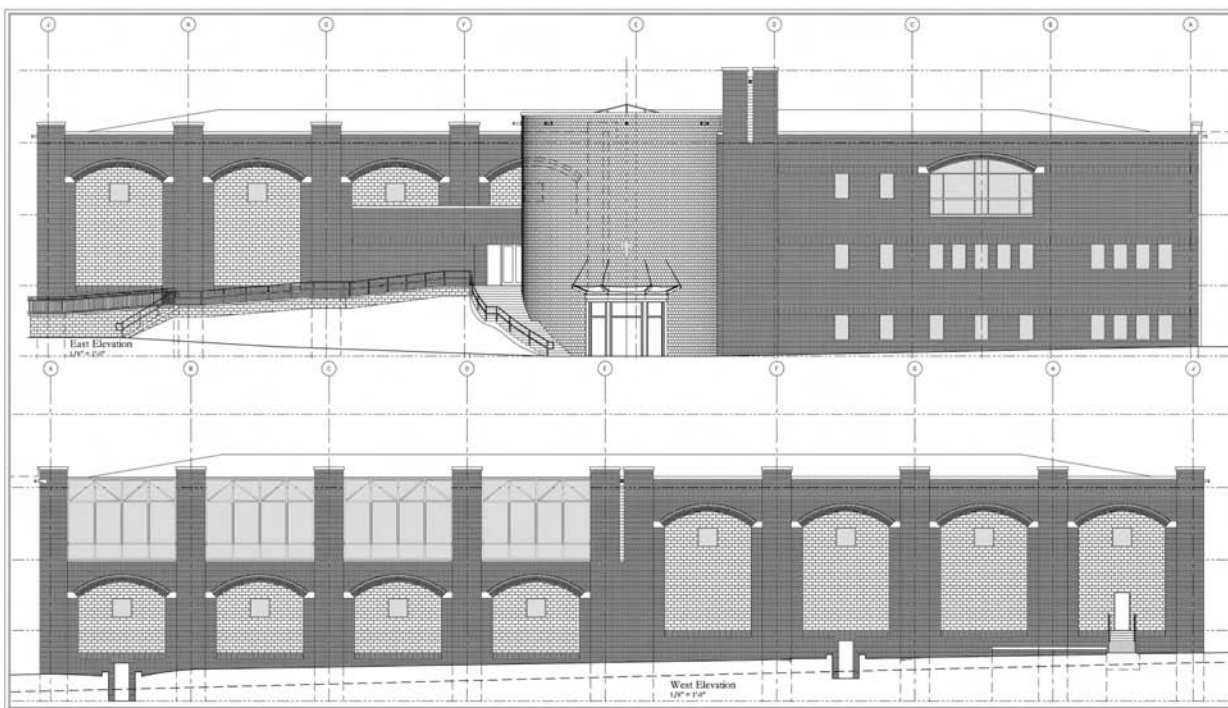
VILLANOVA UNIVERSITY INTERCOLLEGIATE ATHLETICS & RECREATION FACILITY EAST & WEST ELEVATIONS
