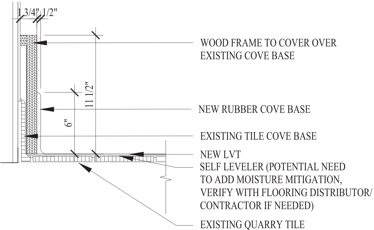
NEW FLOORING TRIM DETAIL
