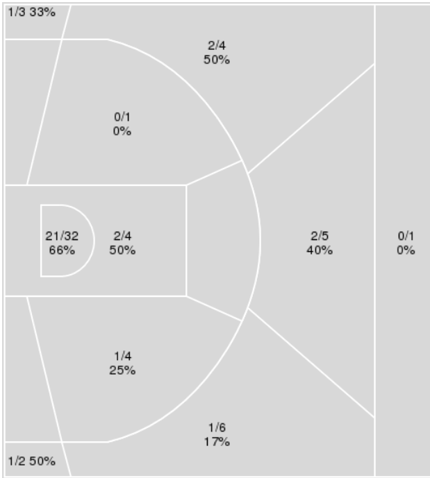
Grand Canyon
