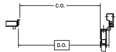
HORIZONTAL CLEAR OPENING (OPAQUE DOOR - ACTIVE LEAF)
