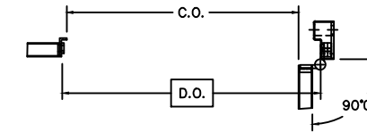
HORIZONTAL CLEAR OPENING (OPAQUE DOOR - ACTIVE LEAF)
