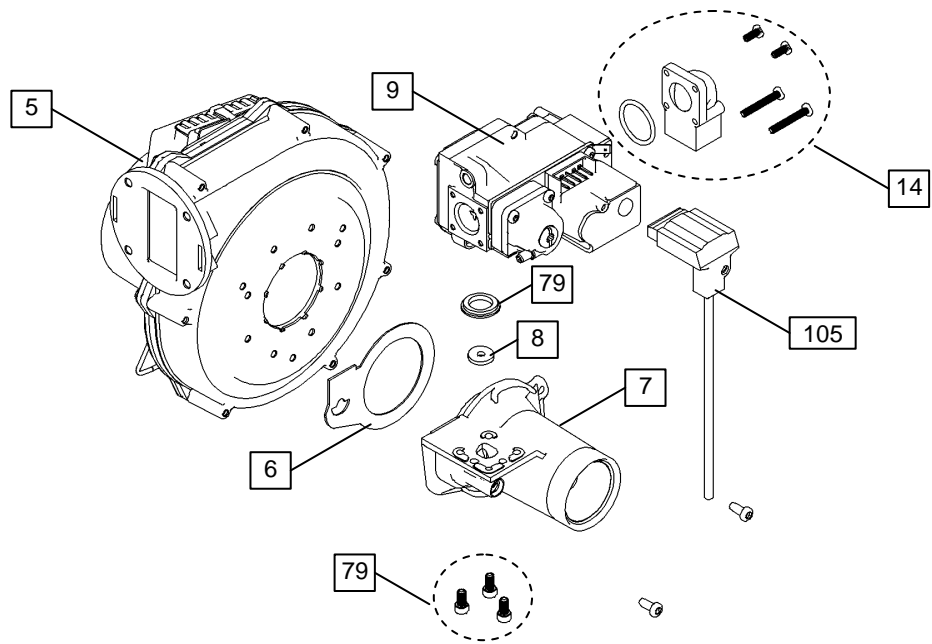
Figure 7-2 Tx200 Gas Valve & Blower Assembly
