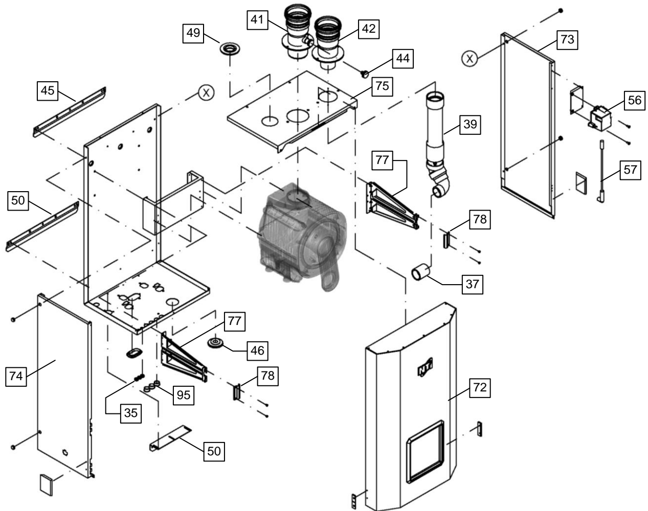
Figure 7-3 Tx Cabinet Cabinet, Vent and Air-Inlet Parts
