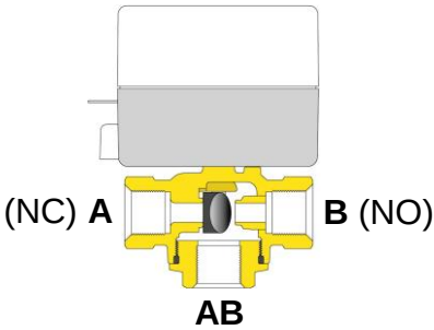
3-way valve with normally closed actuator (Note: 3-way uses only normally closed actuator)
