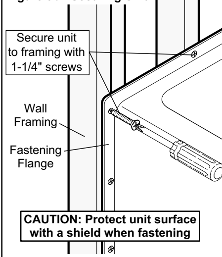
Figure 3b - Securing Unit
