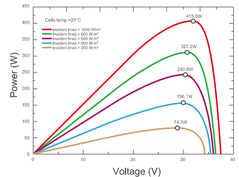
Current-Voltage & Power-Voltage Curves (RMH54-415B1)
