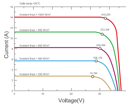
Current-Voltage & Power-Voltage Curves (RMH54-415B1)
