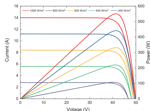
Current-Voltage &amp; Power-Voltage Curve (550W)
