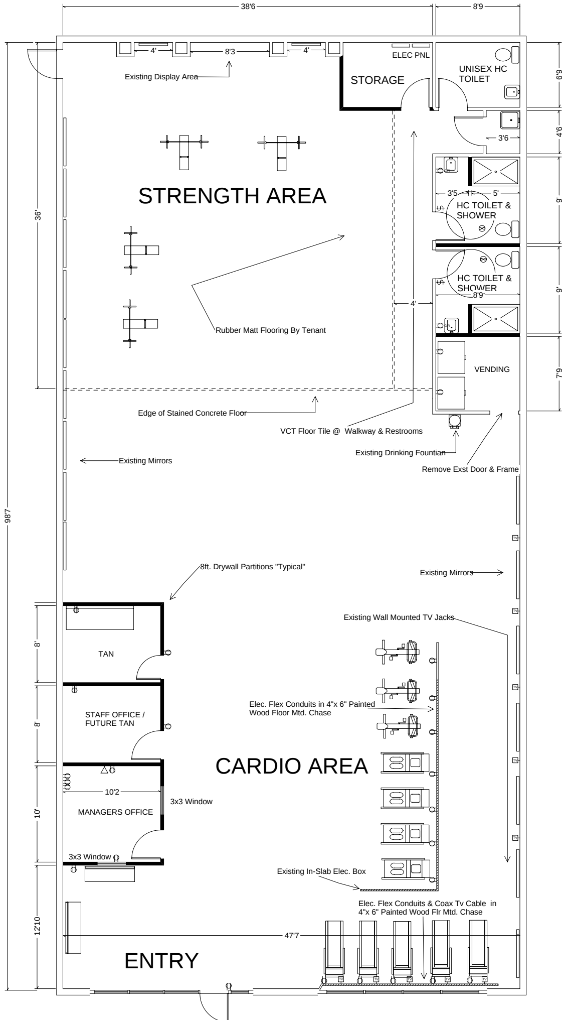
PROPOSED LAYOUT FOR ANYTIME FITNESS; VESTRIDGE GENE R. FOSHEE INC. 4/21/10
