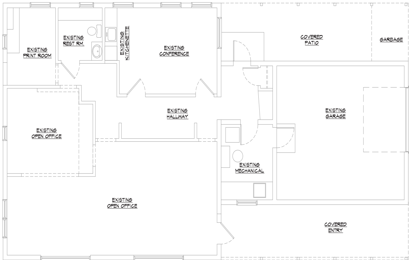
EXISTING FLOOR PLAN 1/8" = 1'-0" TOTAL EXISTING AREA = 1,081 S.F. (INC. GARAGE) OFFICE AREA = 1,451 S.F. GARAGE AREA = 430 S.F.
