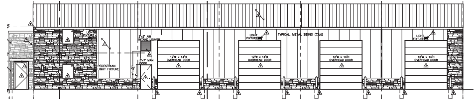
NORTH ELEVATION
