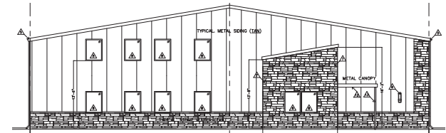
EAST ELEVATION
