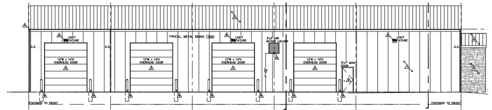
SOUTH ELEVATION
