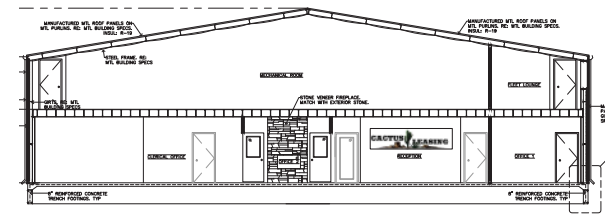
BUILDING SECTION
