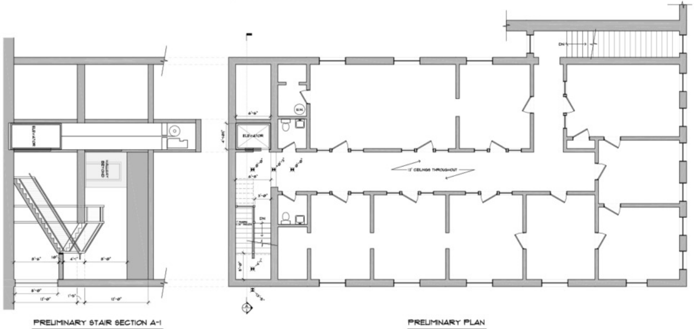
128.5 CHURCH ST. PRELIMINARY LAYOUT 2.19.17 SCALE: 1/8" = 1' @ 11X17 PAPER
