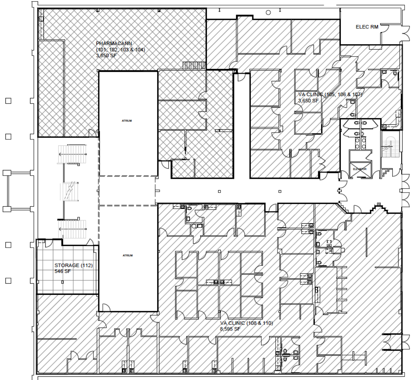
1 1ST FLOOR PLAN A1 1/8"=1'-0"
