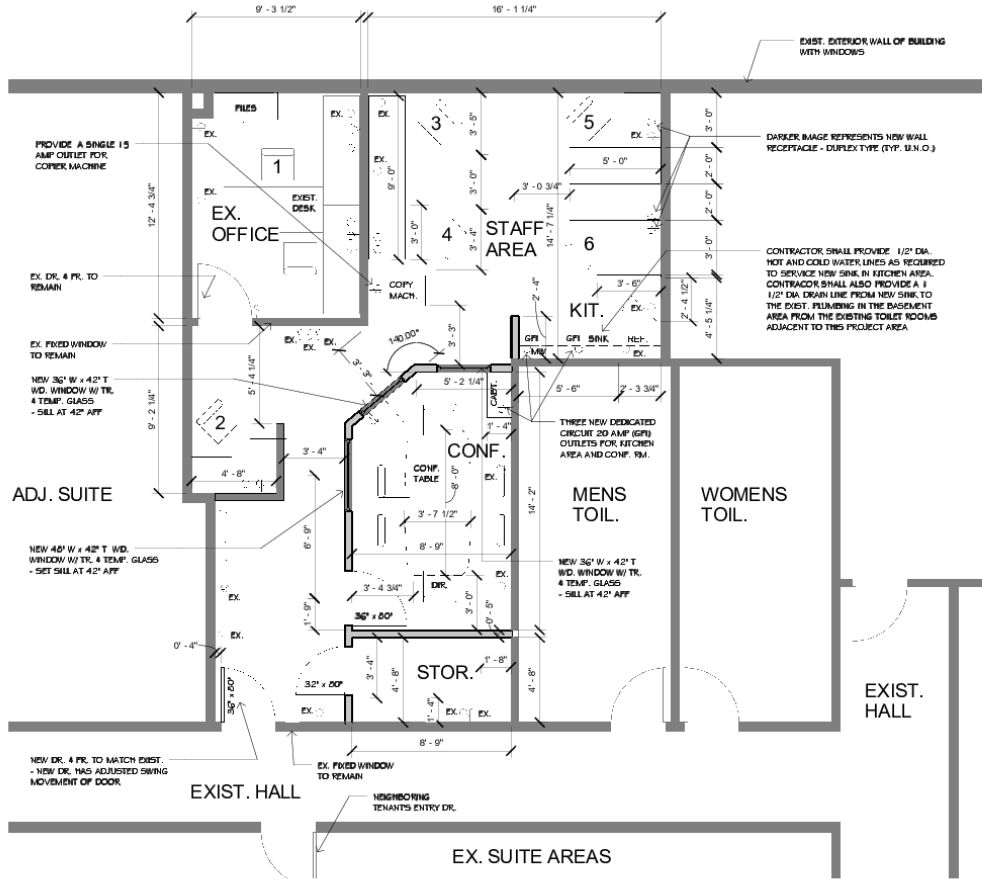
② Level 1 New Floor Plan for Concept A 1/4" = 1'-0"
