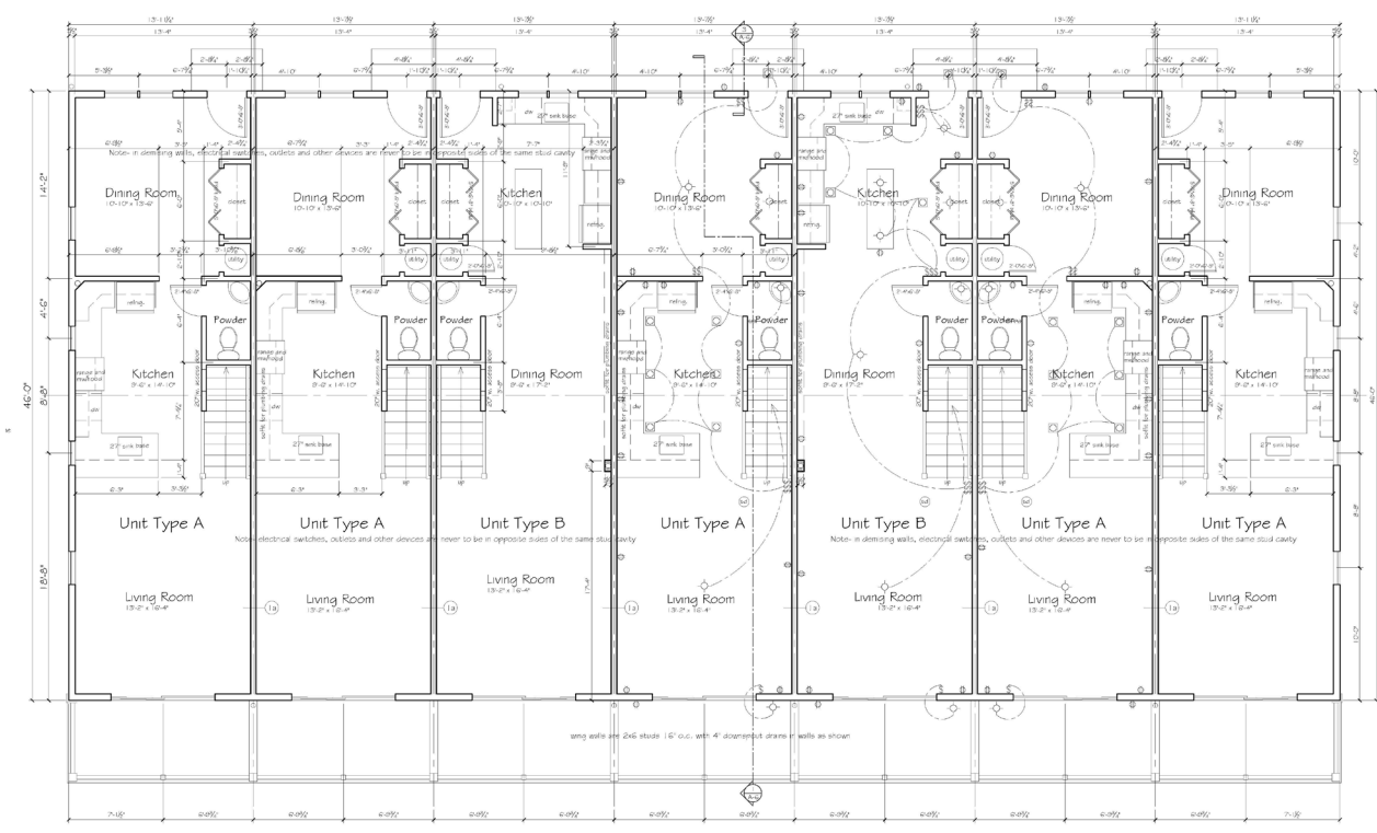
Second Floor Plan Scale: 1/4" = 1'-0"
