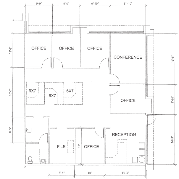
Suite 120 - 1,758 SF
