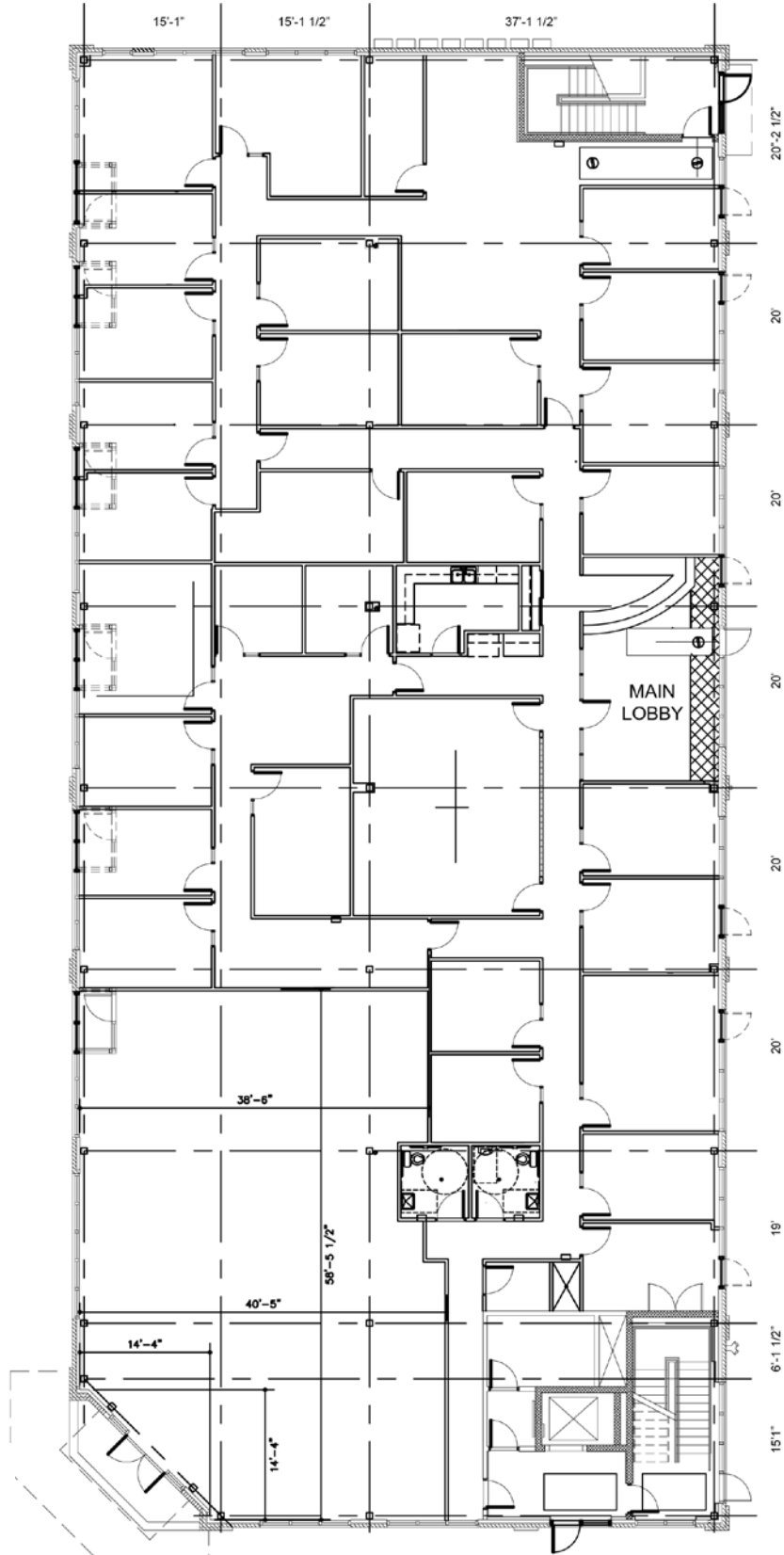
Floor Plan First Floor (as Built)
