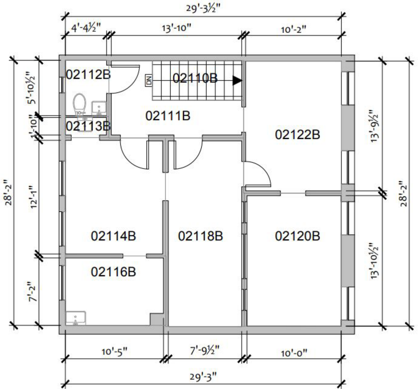
Second Floor
