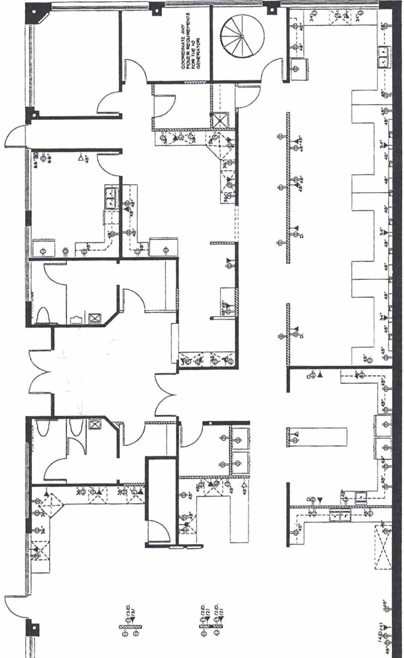
NEW FLOOR PLAN 1/4" = 1'-0"
