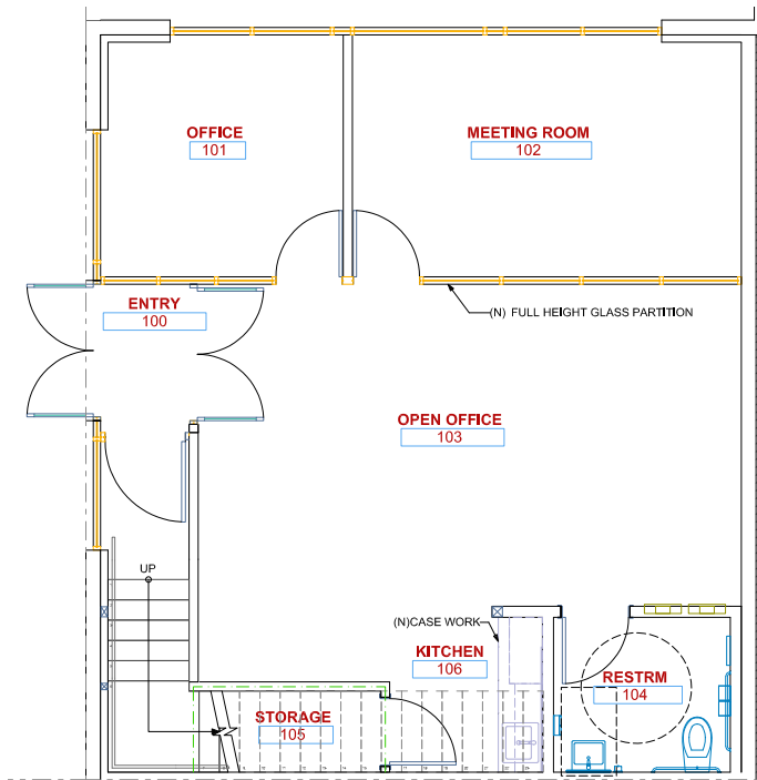
GROUND FLOOR 900±SF
