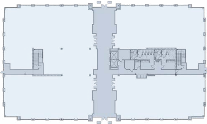
First Floor Plan 22,700 rentable square feet
