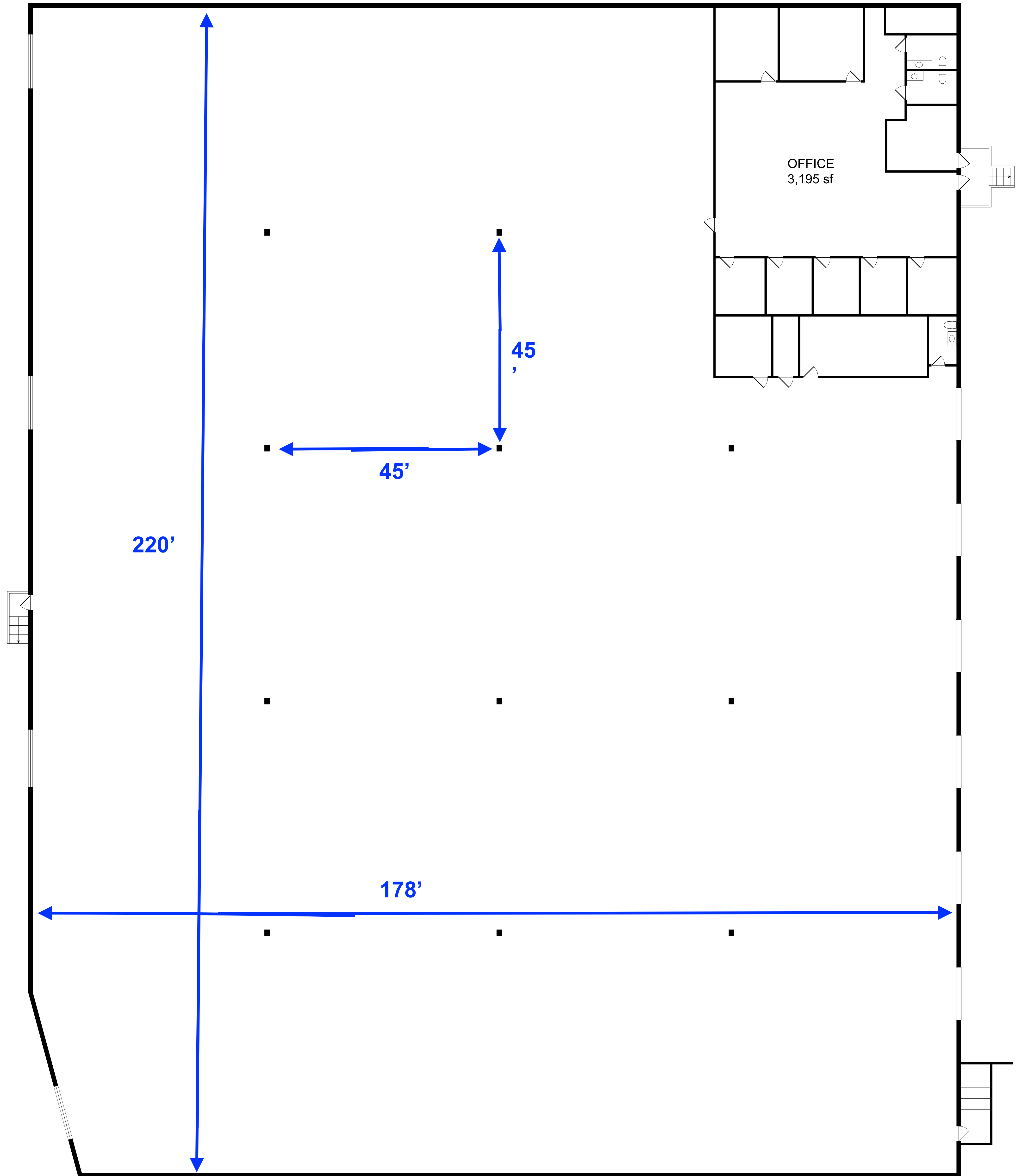
FLOOR PLAN TOTAL SIZE 39,750 SF.
