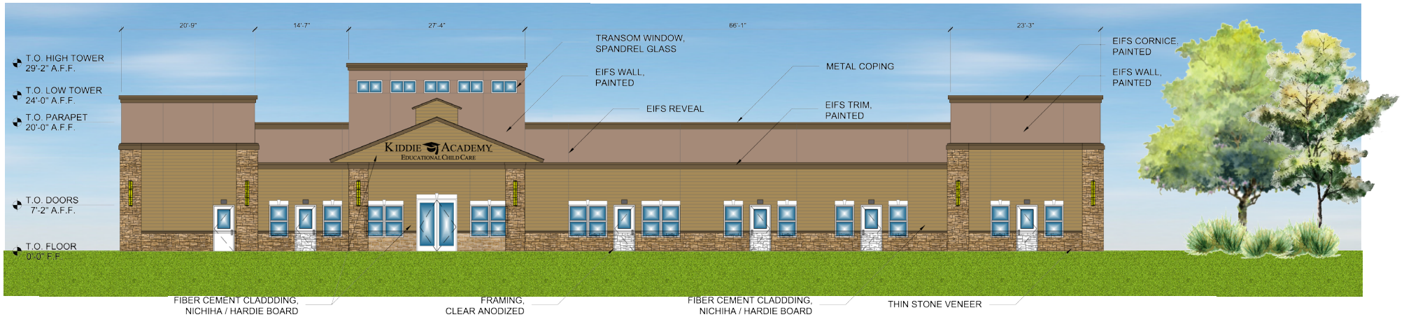
01 NORTH ELEVATION (FRONT)
