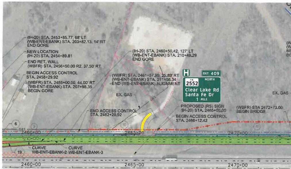
TxDOT Schematic – Whole Property
