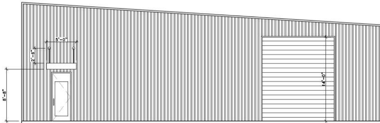
2. EXTERIOR ELEVATION
