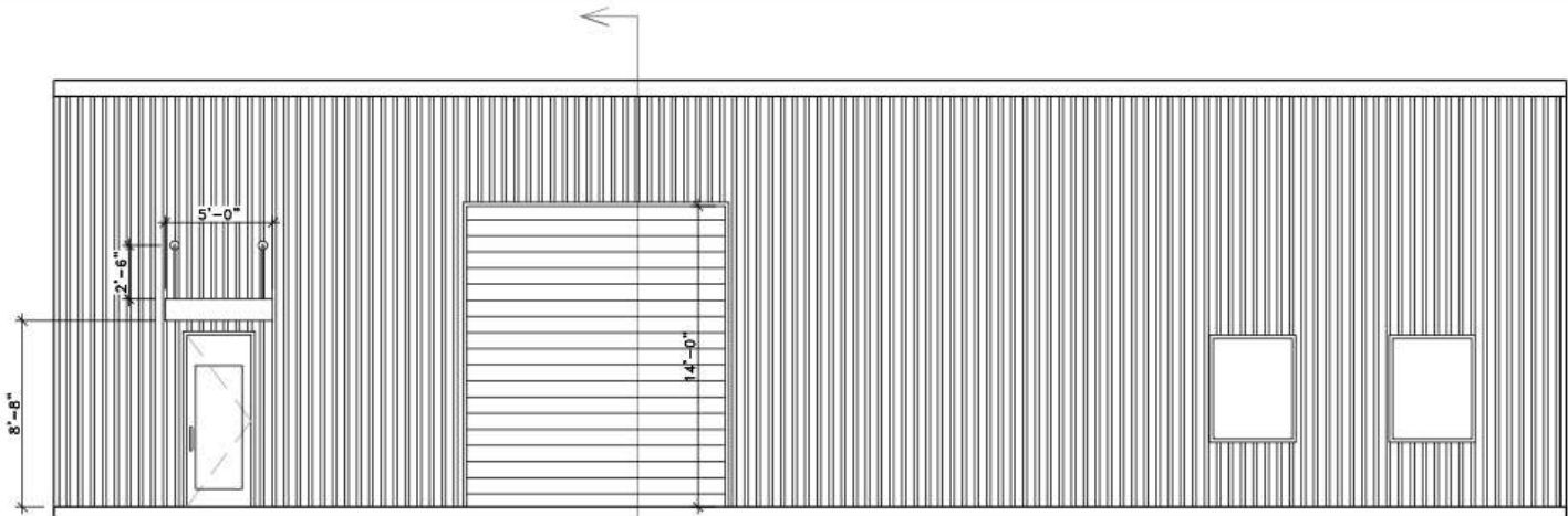
1. EXTERIOR ELEVATION
