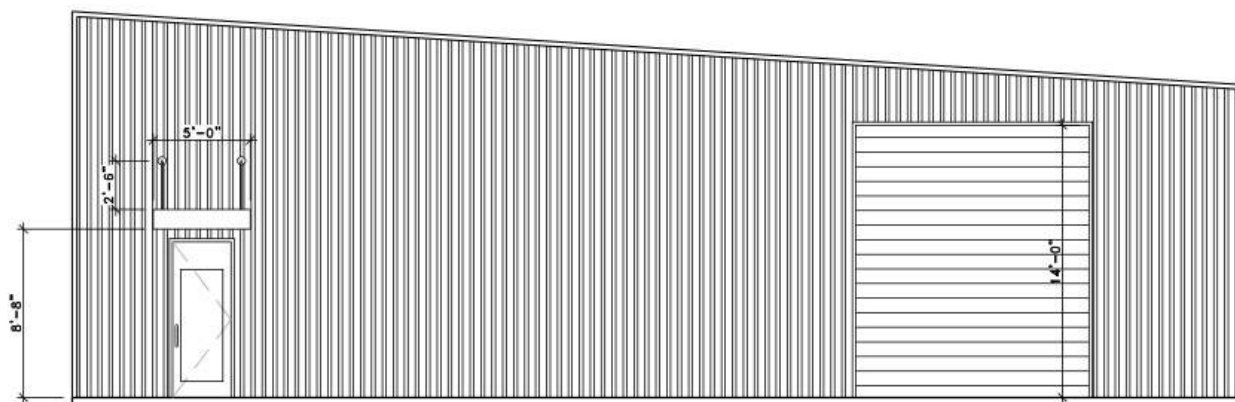
2. EXTERIOR ELEVATION
