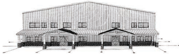
REAR BUILDING ELEVATION SCALE: 1/8" = 1'-0"
