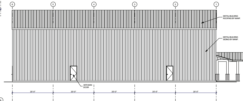
LEFT SIDE BUILDING ELEVATION SCALE: 1/8" = 1'-0"
