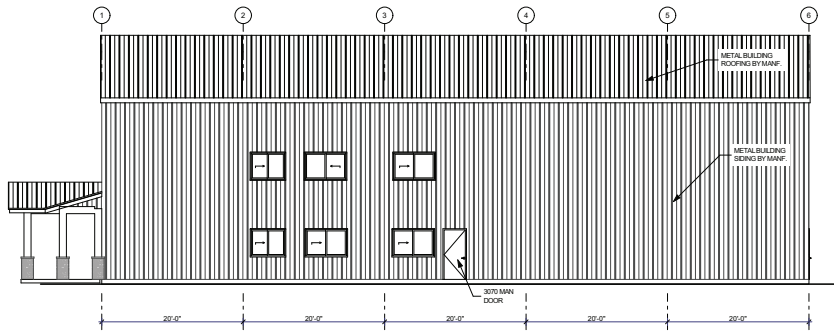
RIGHT SIDE BUILDING ELEVATION SCALE: 1/8" = 1'-0"
