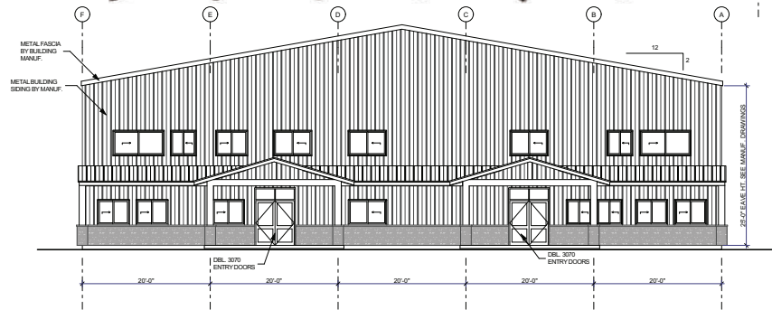
FRONT BUILDING ELEVATION SCALE: 1/8" = 1'-0"
