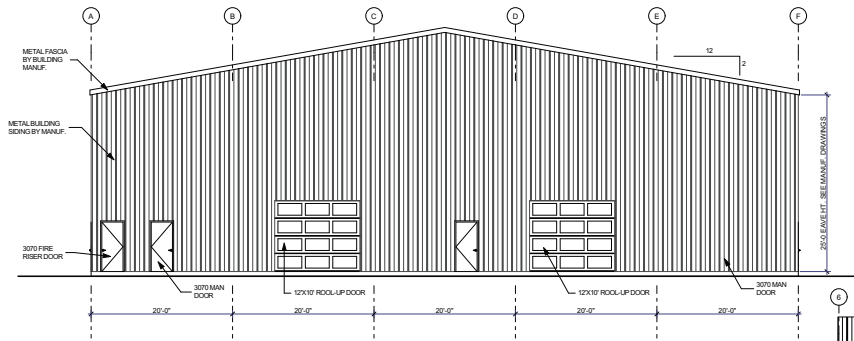
REAR BUILDING ELEVATION SCALE: 1/8" = 1'-0"
