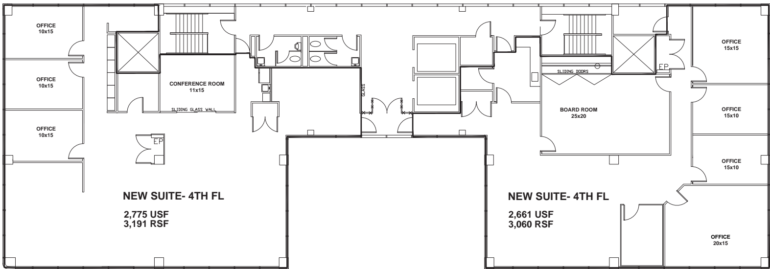
4TH FL PLAN - TWO SEPARATE SUITES
