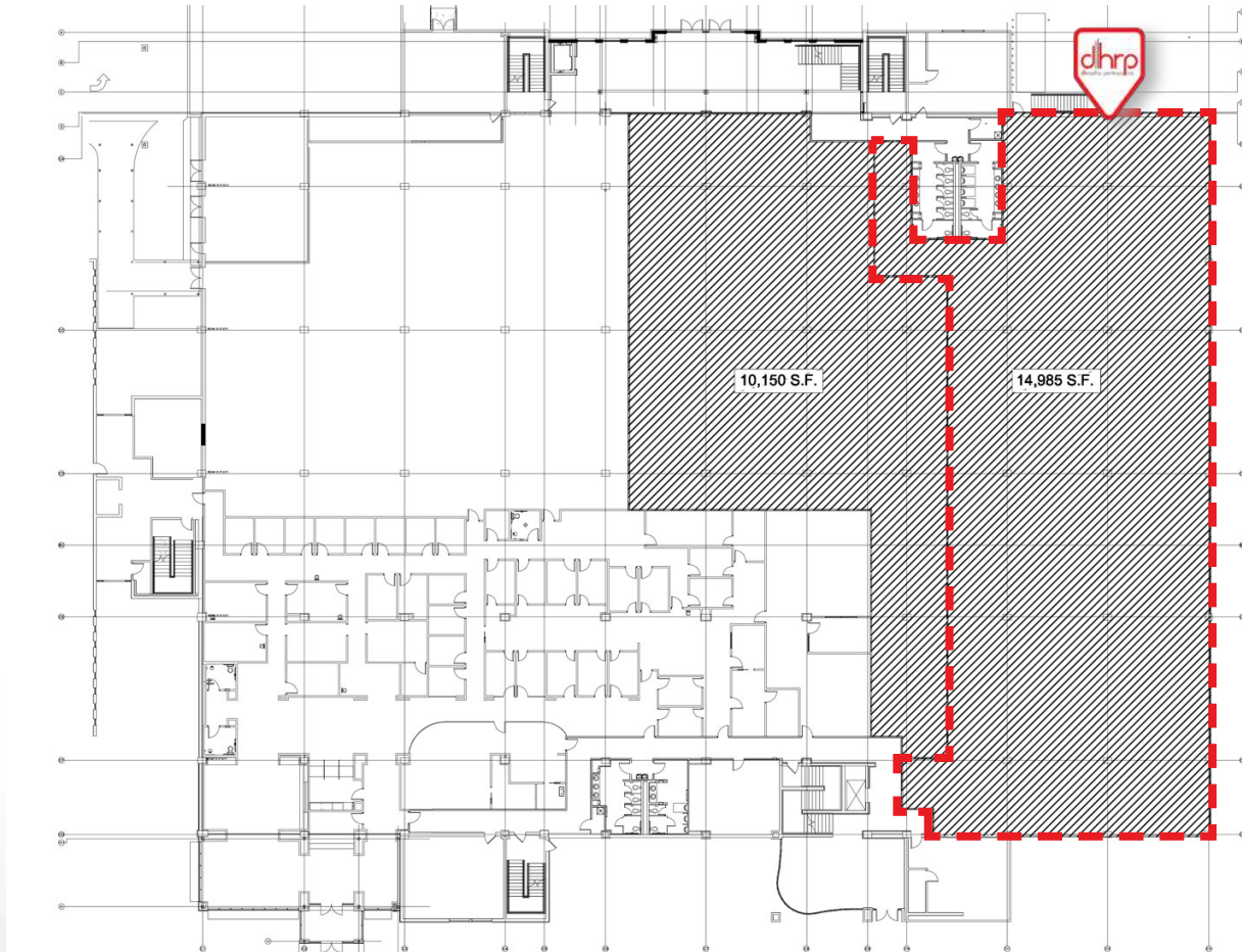
FIRST FLOOR (FLOOR PLAN)
