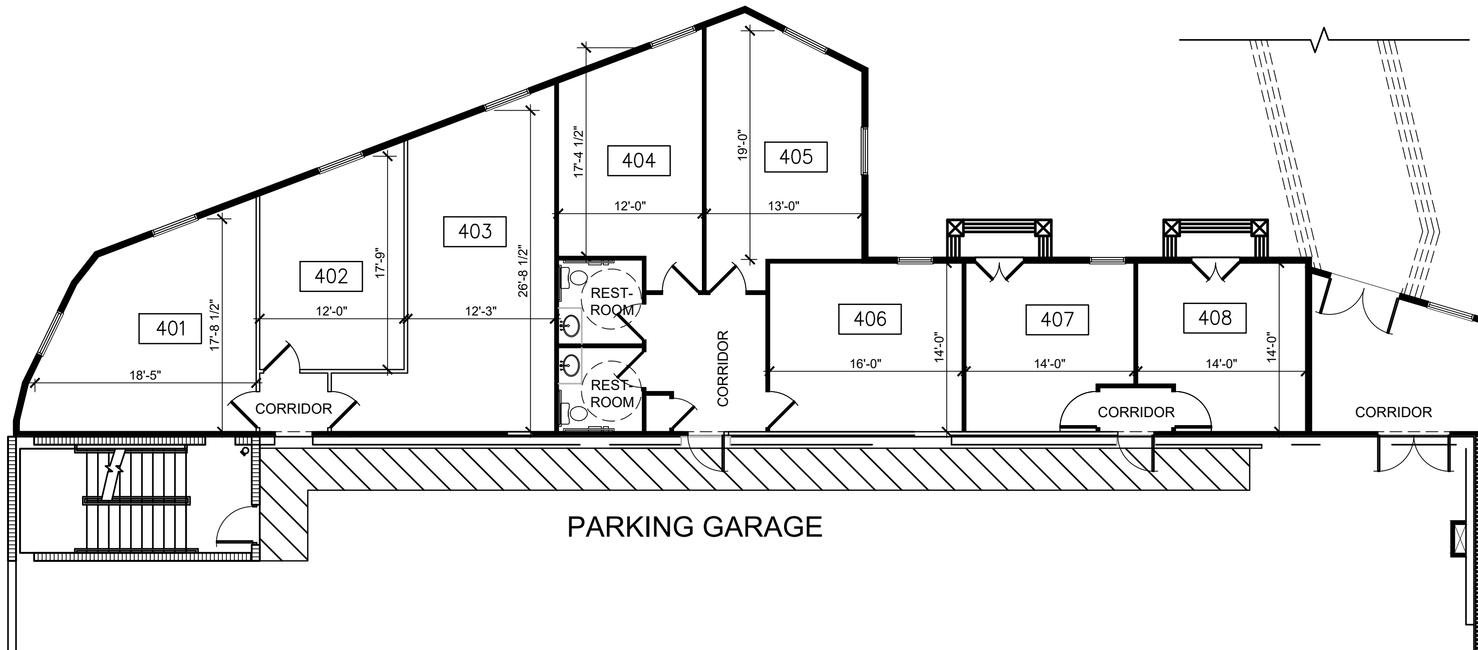
01 Fourth Floor Office Plan SCALE: 1/8" = 1'-0"
