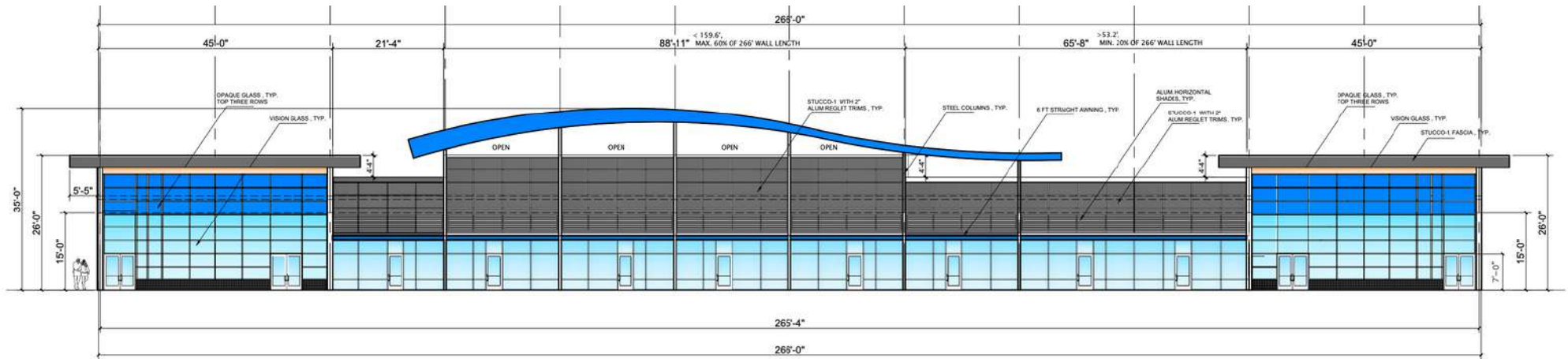
NORTH ELEVATION BUILDING-1 3/32"=1'-0"
