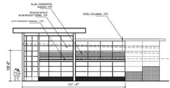
WEST ELEVATION 3/32"=1'-0"
