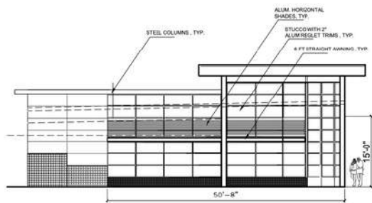
EAST ELEVATION 3/32"=1'-0"
