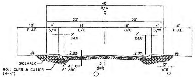
TYPICAL DETAIL A LOCAL STREET-CUL-DE-SAC (NOT TO SCALE)
