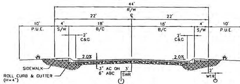
TYPICAL DETAIL A LOCAL STREET (NOT TO SCALE)
