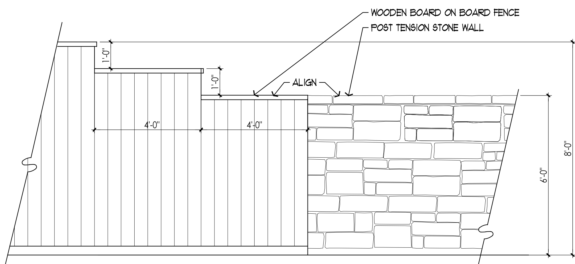
1 DETAIL: WOOD/STONE FENCE TRANSITION NOT TO SCALE
