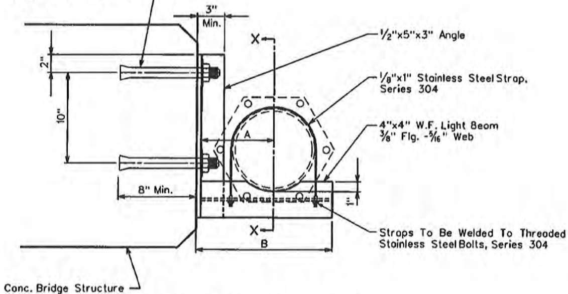
SUSPENSION DETAIL
