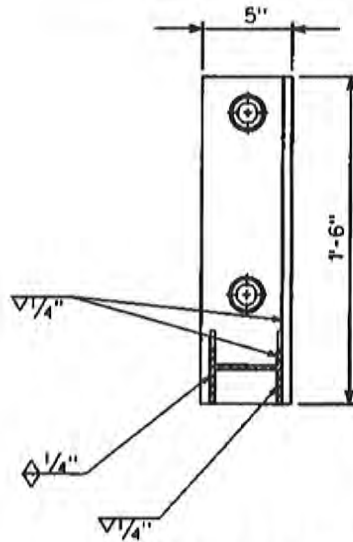
SECTION X-X
