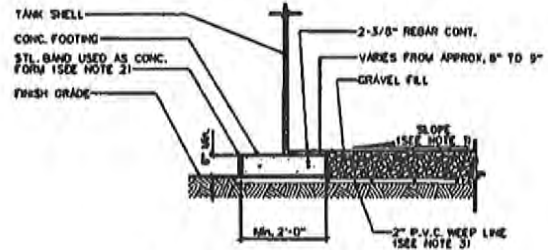
FOUNDATION DETAIL
