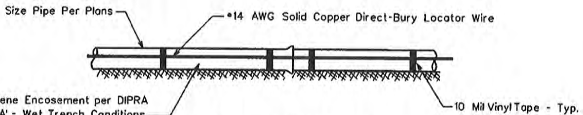
TYPICAL PROFILE VIEW
