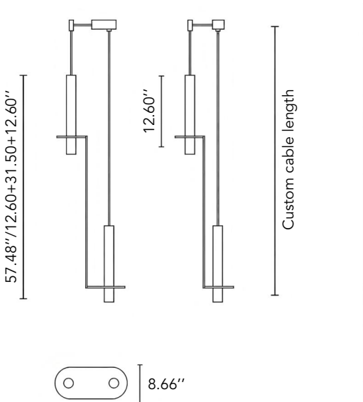
2.6FT/80CM VERTICAL Z SHAPE
