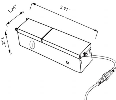
2" 9W-12W Triac / ELV Dimmable 0-10V Dimmable
