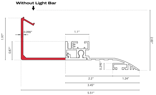
Profile Fixing Bracket
