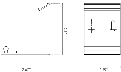
Profile Fixing Bracket
