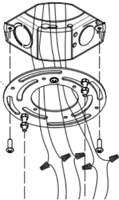
J-box mounting plate
