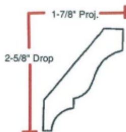
CROWN MOULD M151L 11/16" X 3-1/4"
