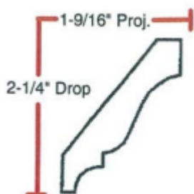
Crown Mould P151L 9/16" X 3-1/4"
