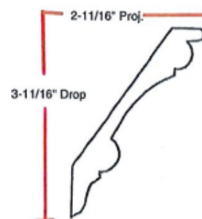
Crown Mould P9923 1/16" X 4-1/2"
