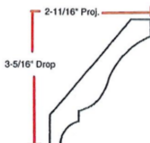
Crown Mould P948L 9/16" X 4-1/4"
