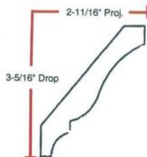
Crown Mould P148L 9/16" X 4-1/4"
