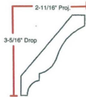
CROWN MOULD KA48 3/4" X 4-1/4"
