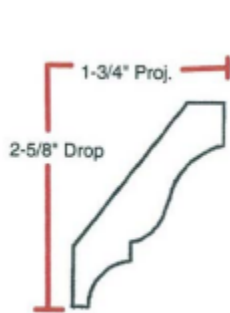
CROWN MOULD KA51 11/16" X 3-1/4"
