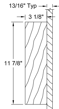
Lock Block Detail w/ Frame
