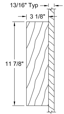
Lock Block Detail w/ Frame
