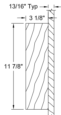
Lock Block Detail w/ Frame
