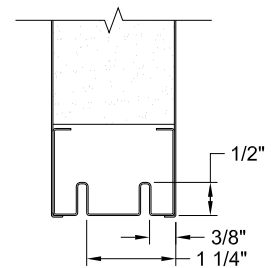
SECTION F-F
