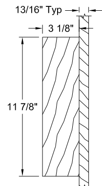
Lock Block Detail w/ Frame
