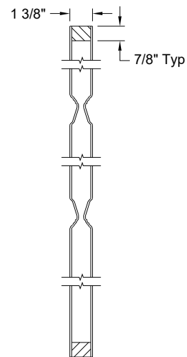
Section A-A Cove & Bead Sticking
