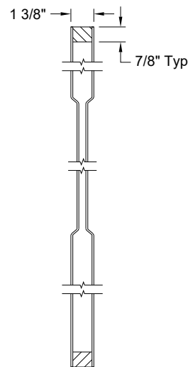
Section A-A Craftsman Sticking
