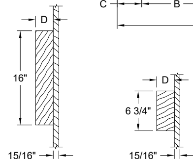
8/0 Lock Block Detail
