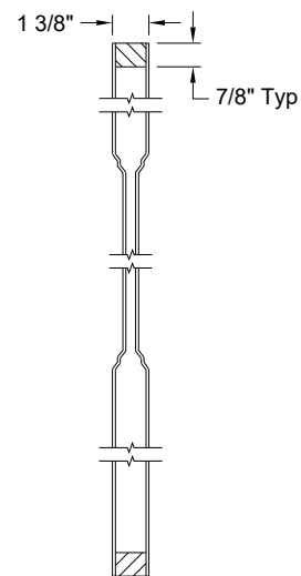
Section A-A Stepped Sticking
