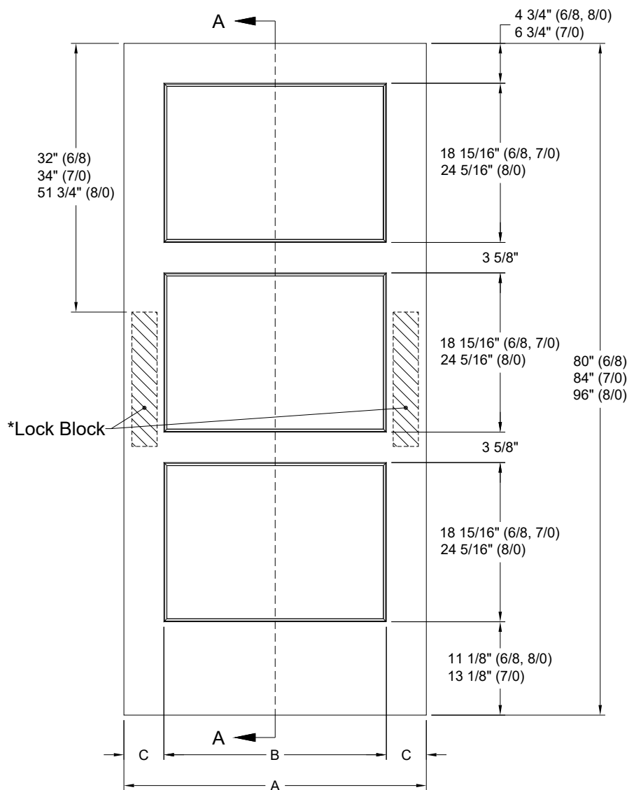
Lock Block Detail
