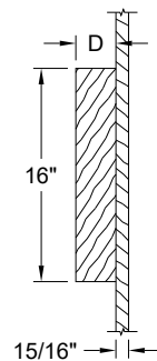
Lock Block Detail
