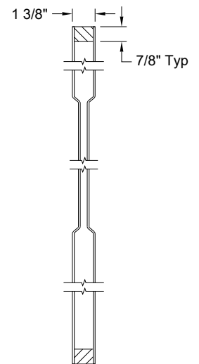
Section A-A Craftsman Sticking
