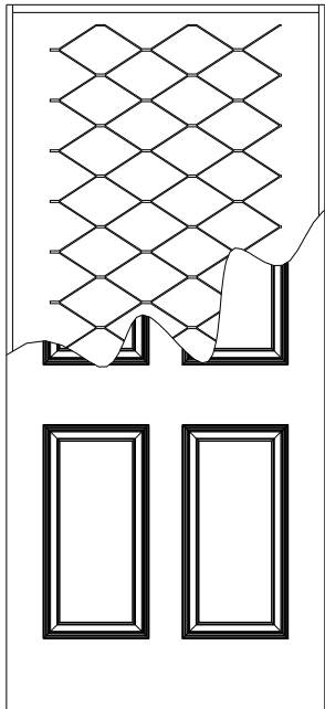
Corrugated Core Wood/MDF or All-Wood Frame
