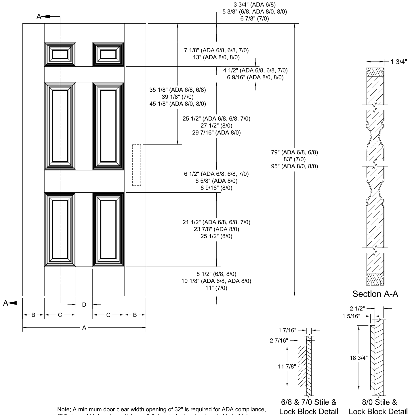
DIMENSION TABLE
