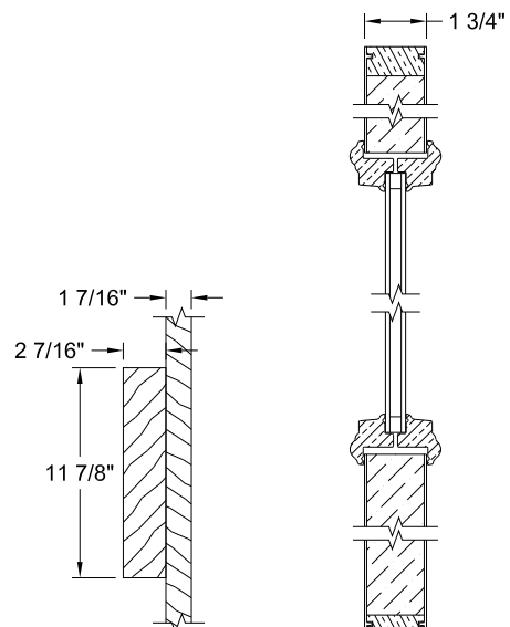
6/8 & 7/0 Stile & Lock Block Detail Section A-A
