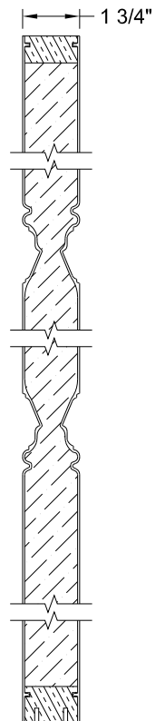
6/8 Stile & Lock Block Detail Section A-A
