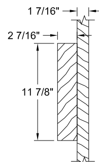
8/0 Stile & 6/8 & 7/0 Stile & Lock Block Detail
