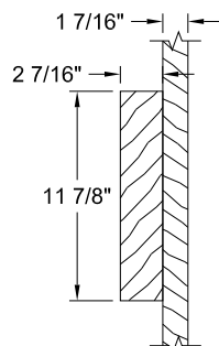
6/8 & 7/0 Stile & Lock Block Detail Section A-A
