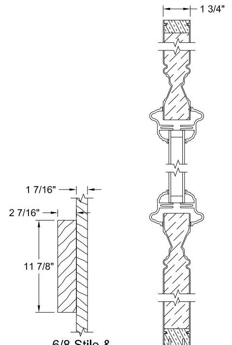
6/8 Stile & Lock Block Detail Section A-A
