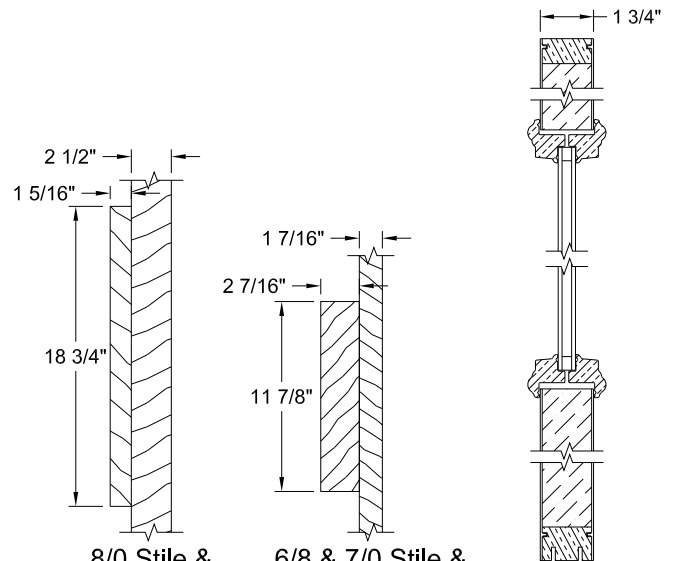
8/0 Stile & Lock Block Detail 6/8 & 7/0 Stile & Lock Block Detail Section A-A
