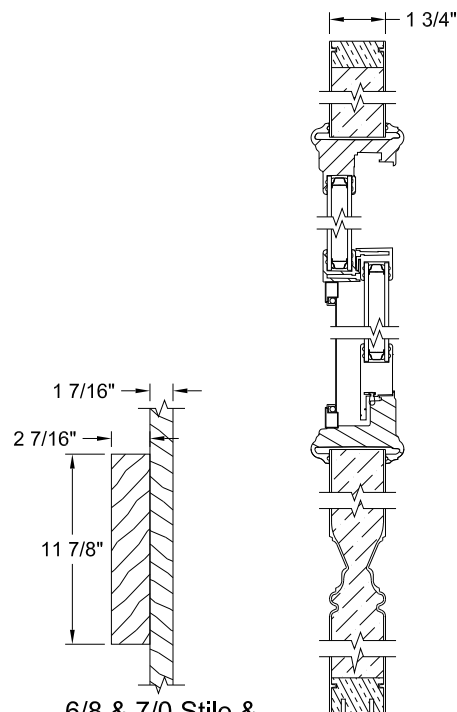
6/8 & 7/0 Stile & Lock Block Detail Section A-A
