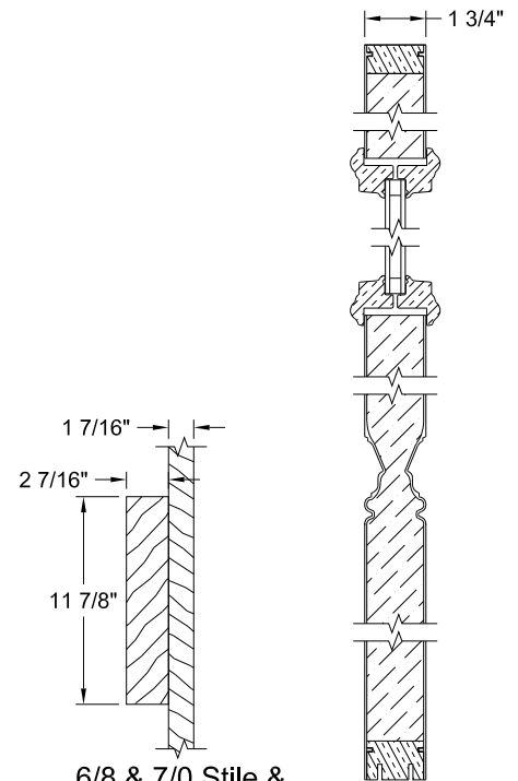
6/8 & 7/0 Stile & Lock Block Detail Section A-A
