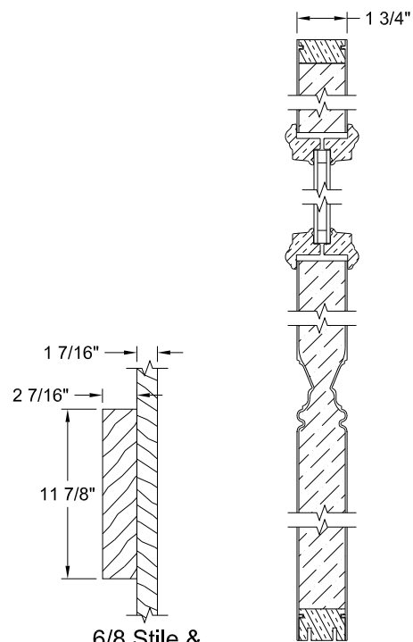
6/8 Stile & Lock Block Detail Section A-A
