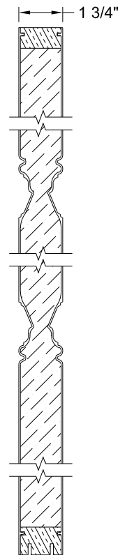
6/8 Stile & Lock Block Detail Section A-A
