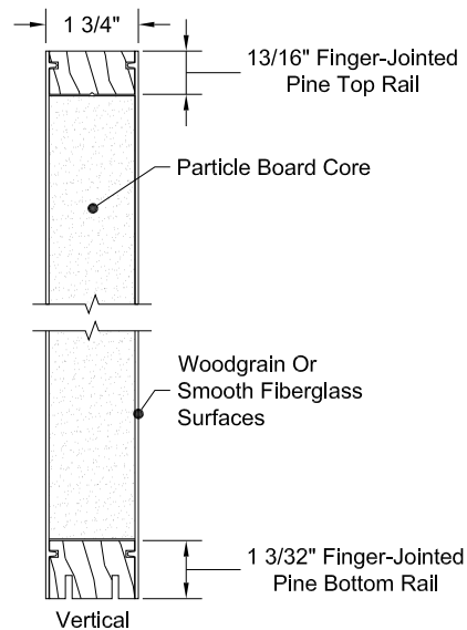
8/0 Sections
