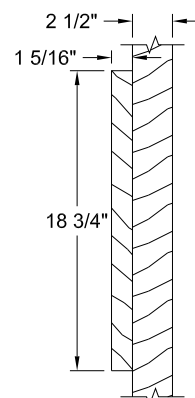
8/0 Stile & 6/8 & 7/0 Stile & Lock Block Detail
