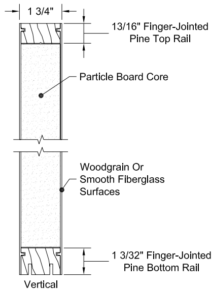
6/8 & 7/0 Sections
