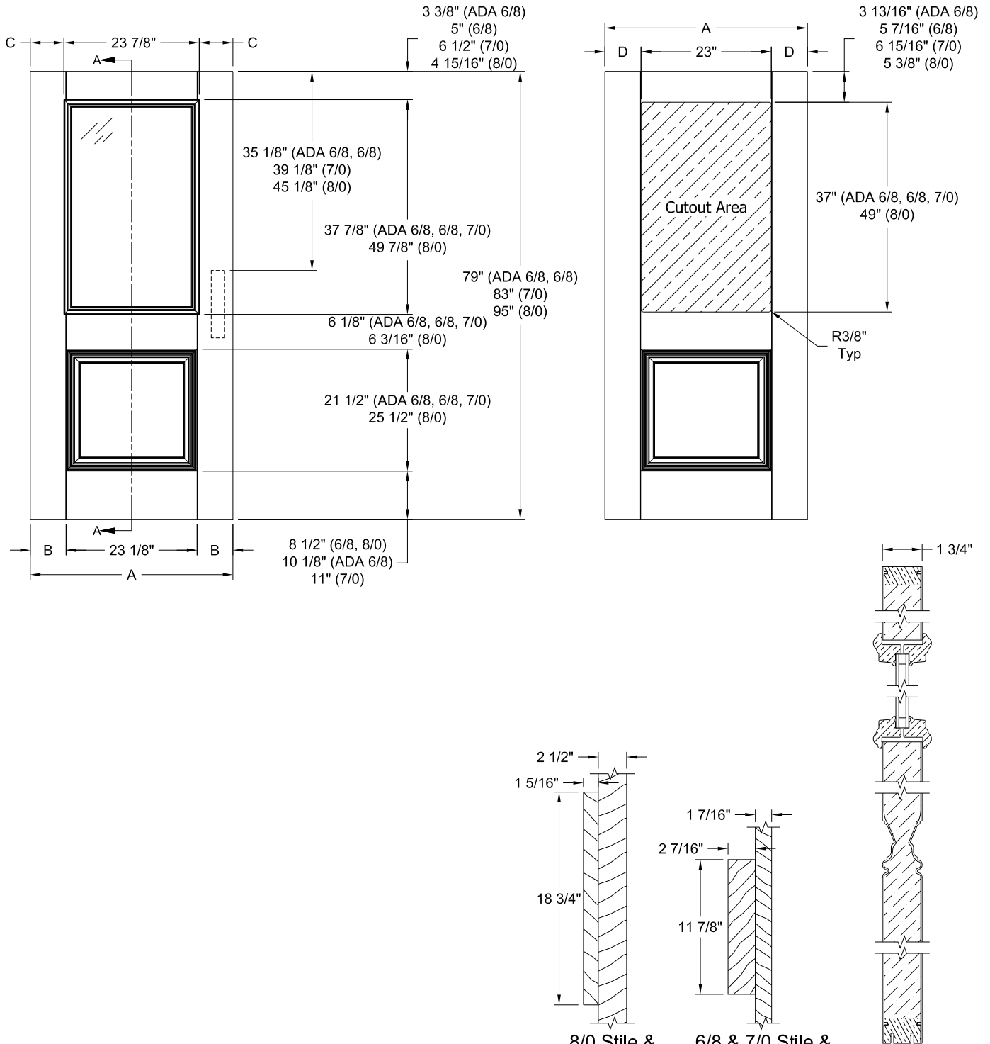
8/0 Stile & 6/8 & 7/0 Stile & Lock Block Detail Lock Block Detail Section A-A
