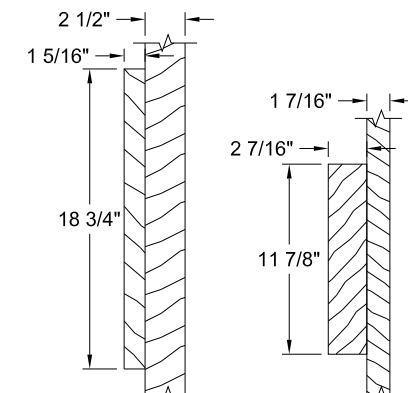
8/0 Stile & Lock Block Detail 6/8 & 7/0 Stile & Lock Block Detail Section A-A
