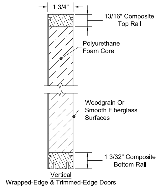
8/0 Sections
