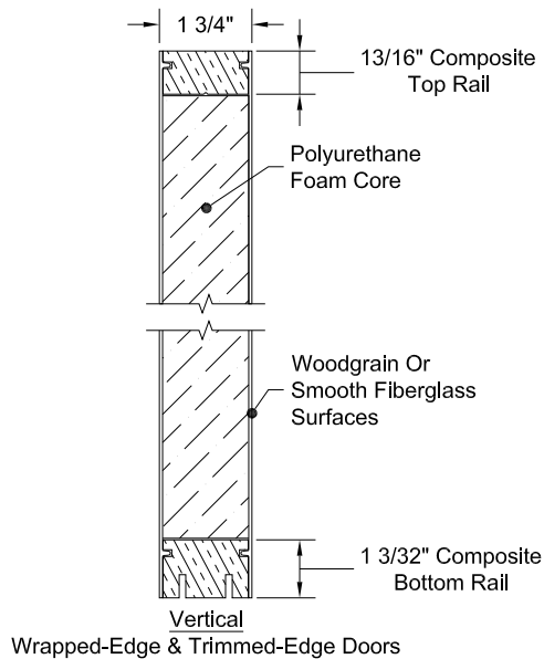
6/8 & 7/0 Sections
