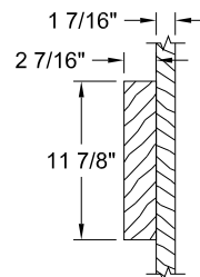
6/8 Stile & Lock Block Detail Section A-A
