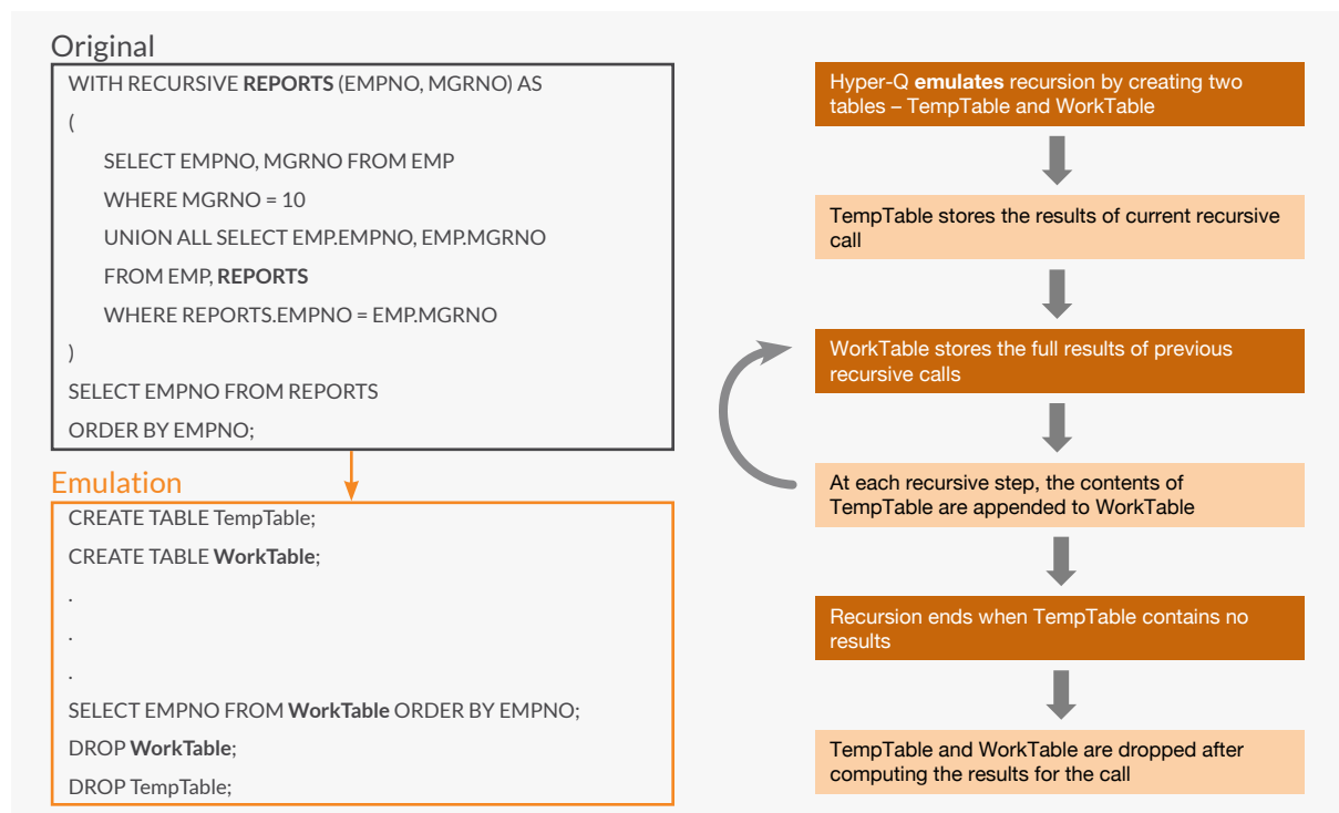
Figure 3. Hyper-Q: Emulating Recursion
