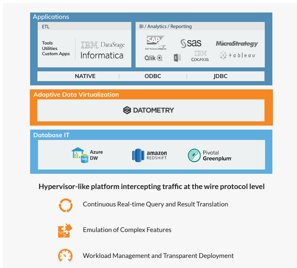
Figure 1. Datometry Hyper-Q: Adaptive Data Virtualization
