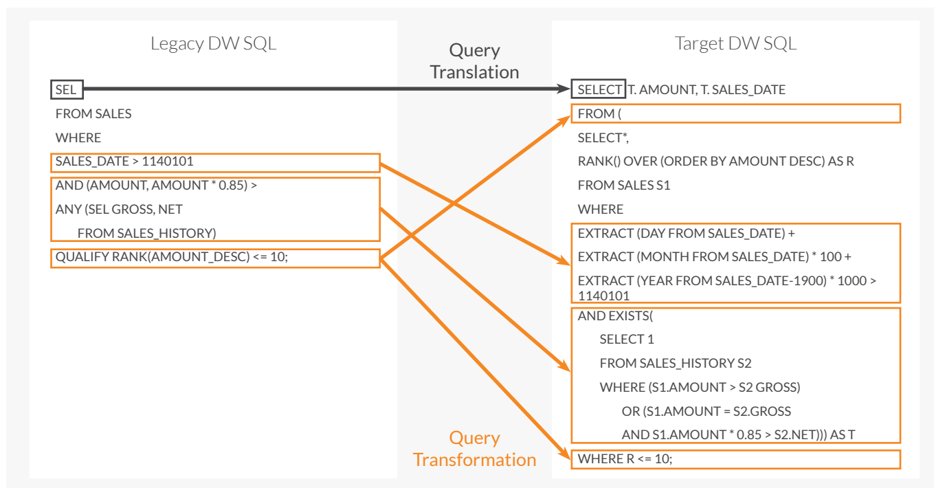
Figure 2. Hyper-Q: Query Translation and Transformation
