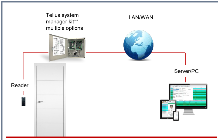
Typical Tellus system topology
