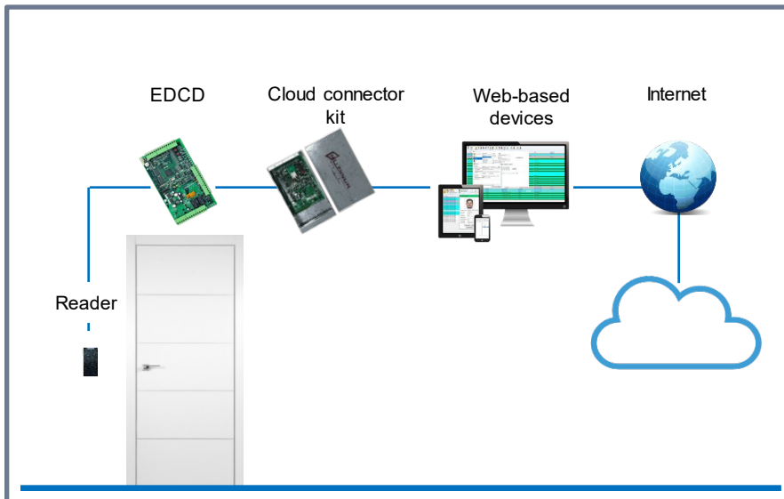
Cloud-hosted system topology
