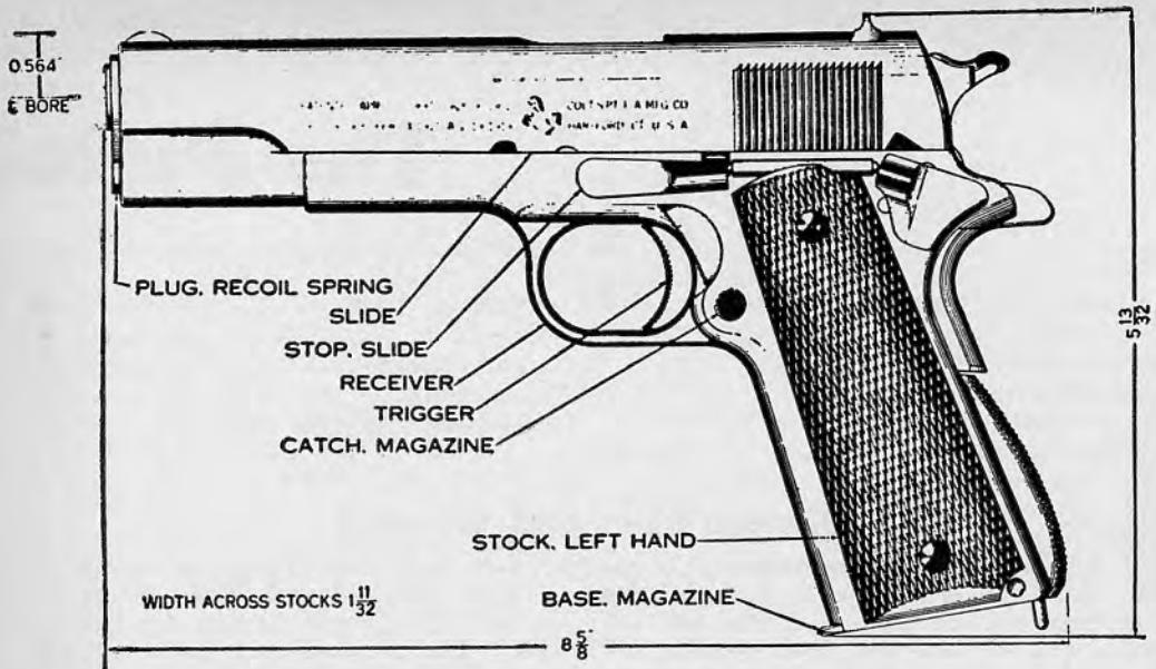
24.1 Basic Nomenclature (Mechanism in Forward Position).
