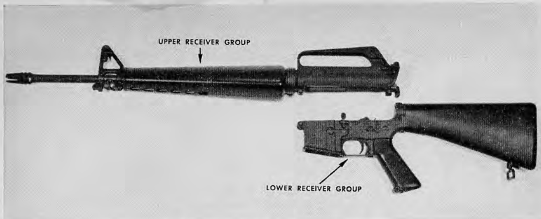
34.5 Upper and lower receiver groups.
