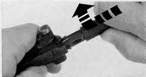
35.13 Unseating extractor.
