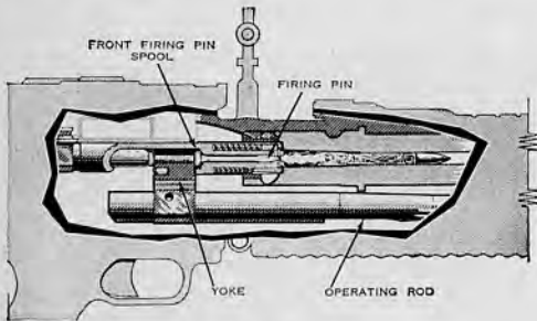
36.29 Firing.
