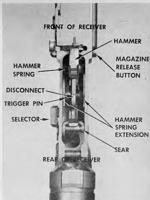
34.25 Position of the hammer spring in the receiver.
