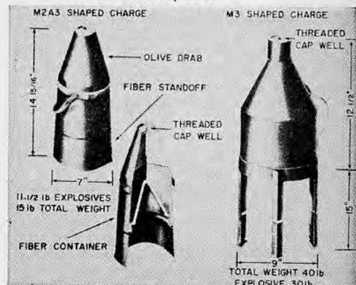
29.14 Shaped Charge M2A3 and M3.
