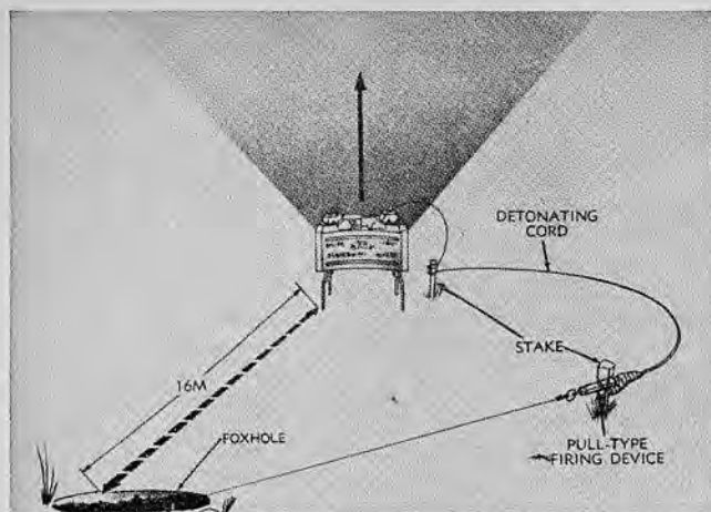
29.29 M18A1 Anti-personnel Mine set up for controlled firing.
