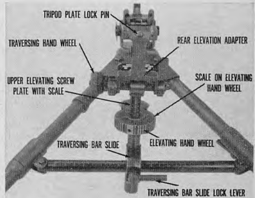
36.34(c) Traversing and elevating mechanism mounted on the M122 tripod mount.
