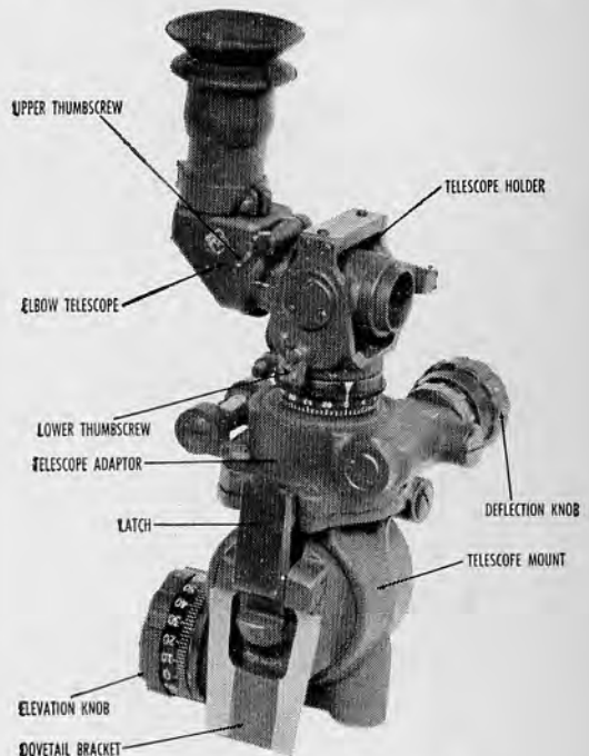
Fig. 30.9(2) Rear view.
