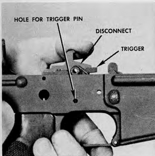
34.21 Removing the trigger and disconnect.
