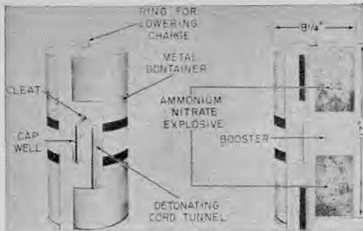
29.15 Ammonium nitrate cratering charge.
