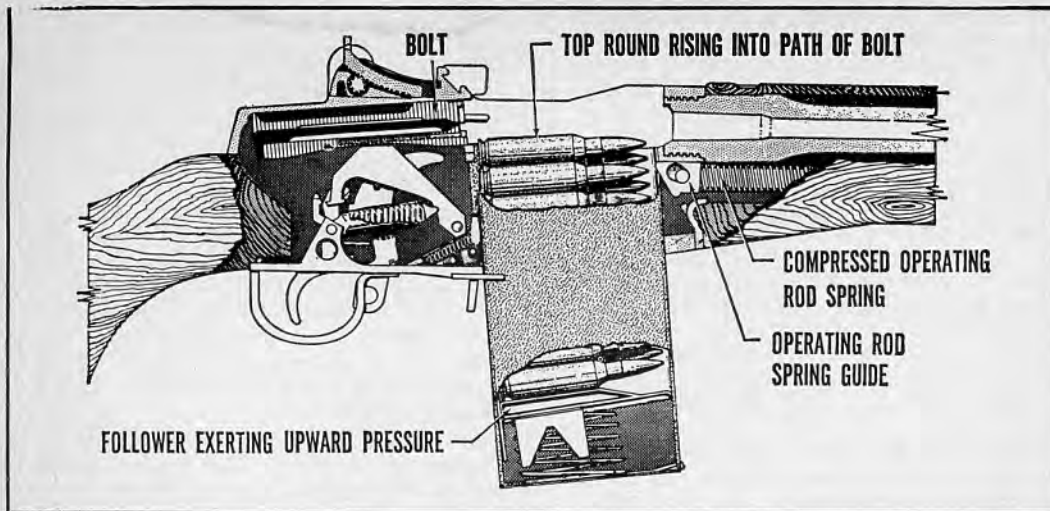
35.23 Feeding.
