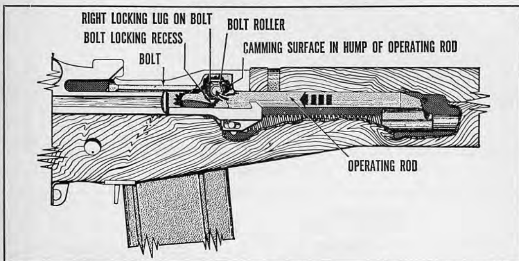
35.28 Unlocking.
