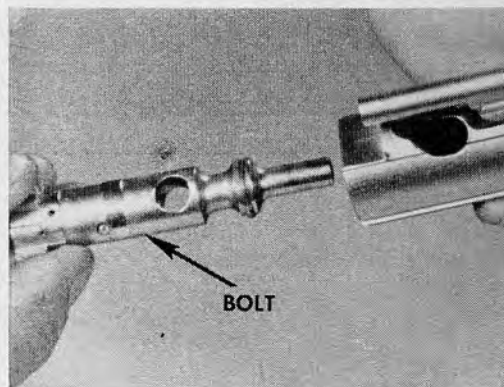
34.12 Removing the bolt from the bolt carrier.
