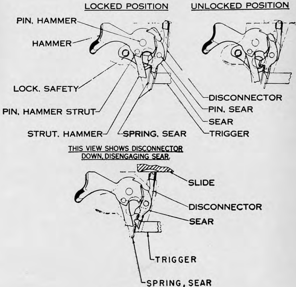
24.8 Safety Lock Mechanism.
