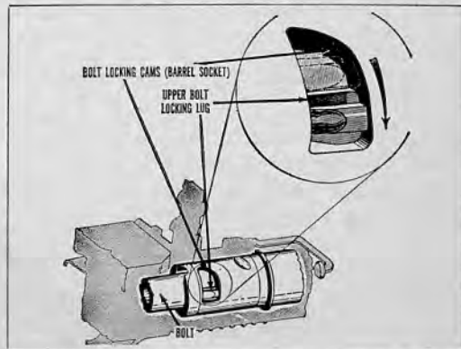
36.28 Locking (upper bolt locking lug rotating clockwise in bolt locking cam in barrel socket).
