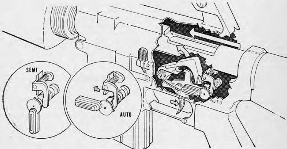
34.36. Automatic sear.
