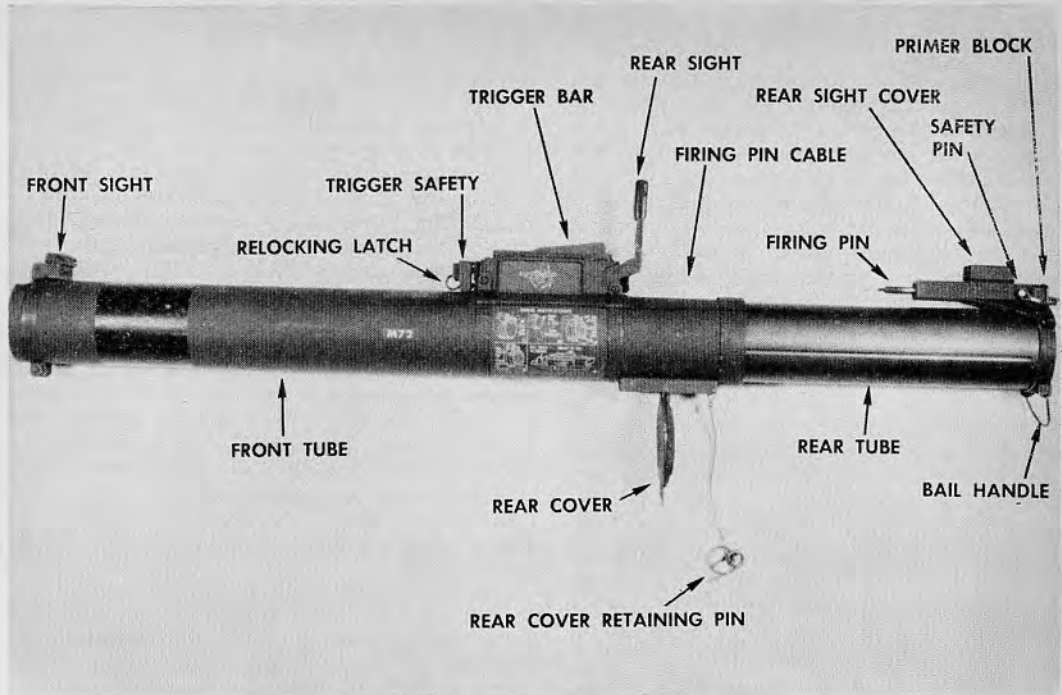
33.5 Outside nomenclature, open position.
