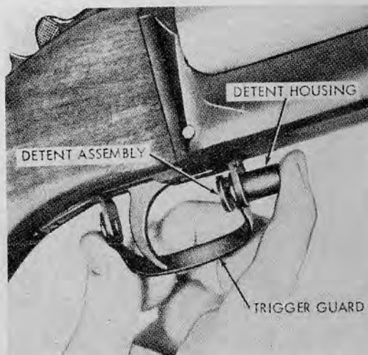
37.12 Operating the trigger guard detent assembly.
