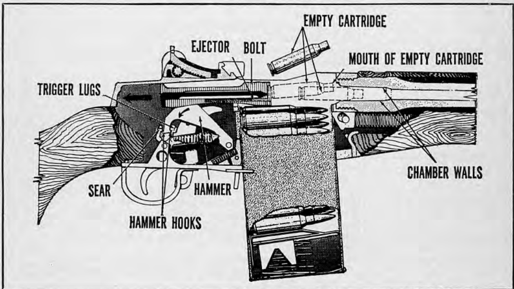
35.30 Ejecting and cocking.
