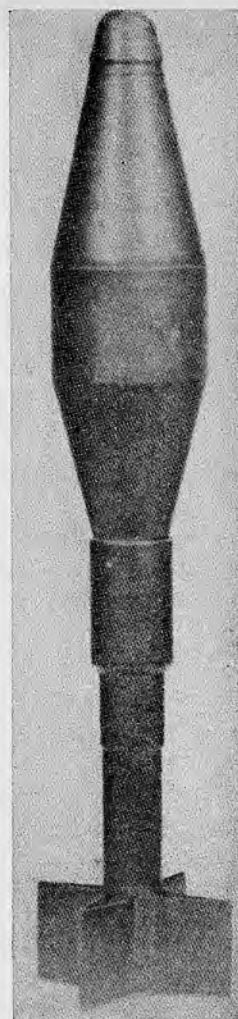
Figure 28.7. M31 HEAT rifle grenade.
