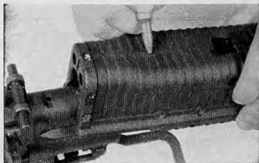
36.20(e) Press down on the cartridge, releasing the forearm latch. Raise the rear of the forearm slightly and remove it to the front.
