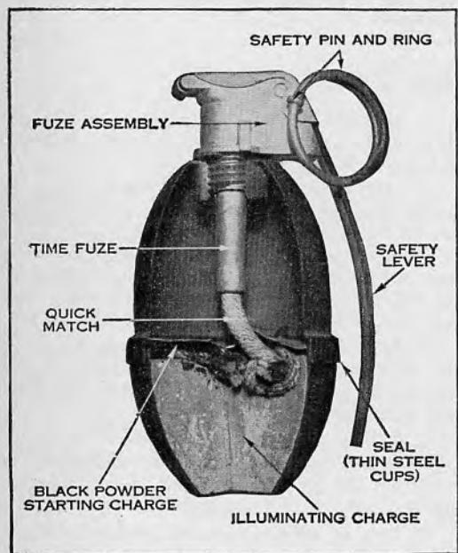
25.3 Illuminating Grenade MK2.
