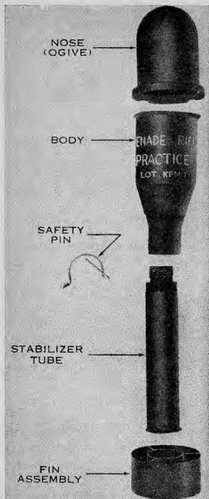
Figure 28.5. M11A4 practice rifle grenade.
