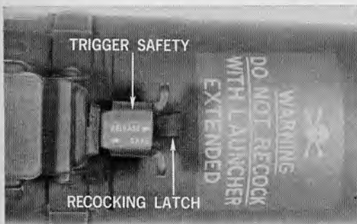
33.7 Location of trigger safety and recocking latch on outer tube.
