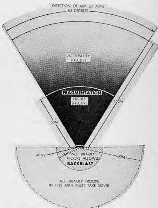
29.28 Casualty area, Anti-personnel Mine M18A1.
