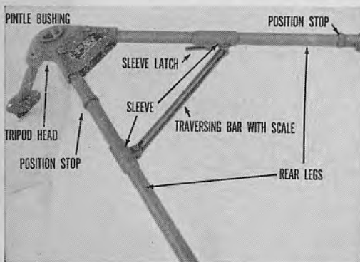
36.34(b) M122 tripod mount without pintle, and without traversing and elevating mechanism.
