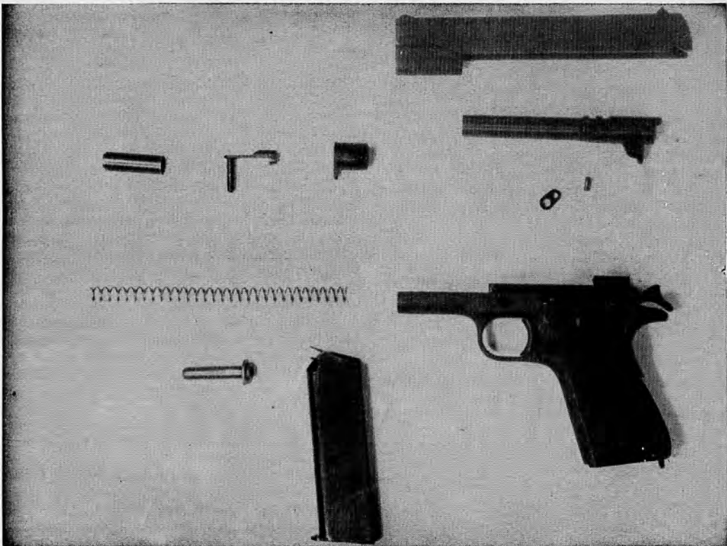
24.6 Field Stripping (Completed).
