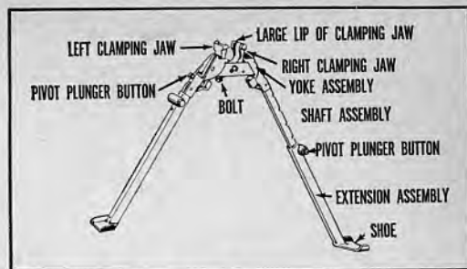
35.41 Rifle Bipod M2, as viewed from the rear.
