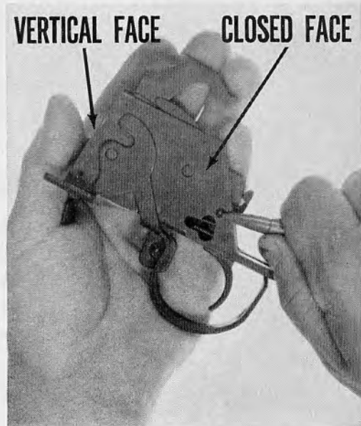
35.9(1) Unseating the trigger pin.
