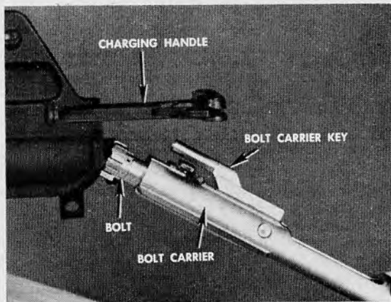
34.7 Removing the bolt carrier from the upper receiver.
