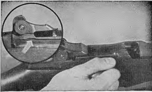
32.6(1) Pull back and up on the operating rod handle until it engages in the dismantling notch.
