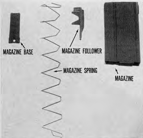
35.16 Parts of the magazine.
