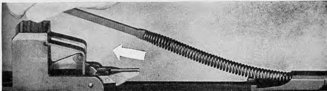
32.5(3) Withdraw follower rod and operating rod spring toward butt of rifle.
