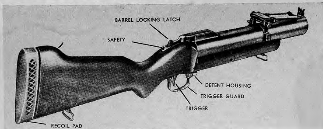
37.1 Grenade launcher M79, right rear view.
