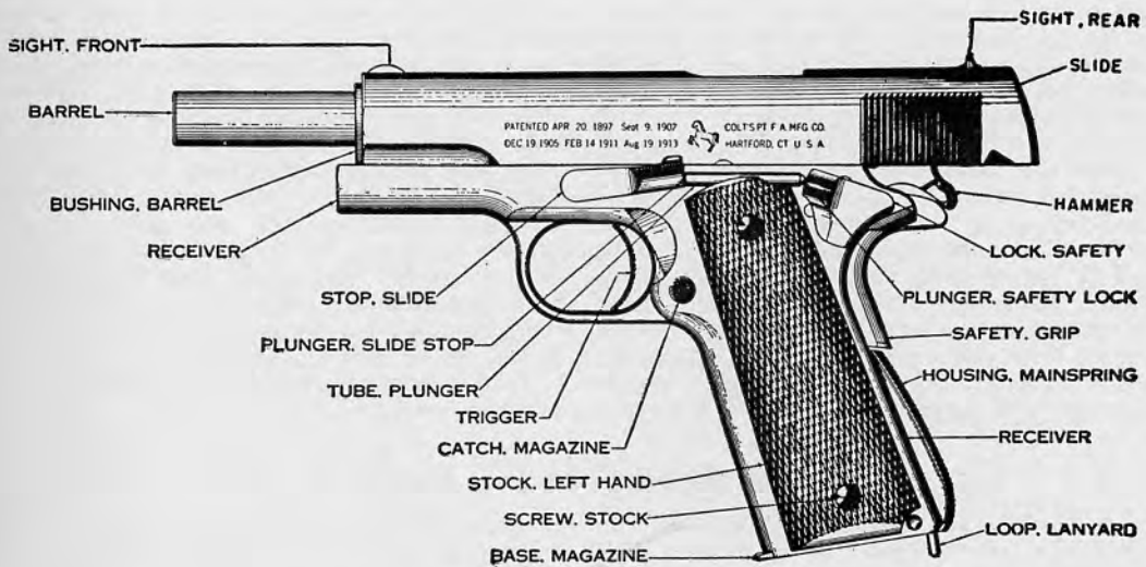
24.2 Basic Nomenclature (Mechanism in Recoil Position).
