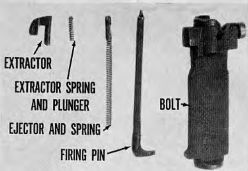
35.14 Parts of the bolt in the order of disassembly.
