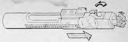
34.34 Locking
