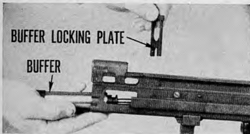
36.5(a) Press in with the palm against the exposed buffer group and remove the buffer locking plate from the top of the receiver.
