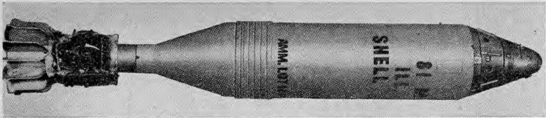
Fig. 30.19(2). Illuminating shell, M301, with time fuze, M84.
