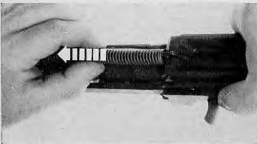
35.6(1) Removing operating rod spring and operating rod spring guide.
