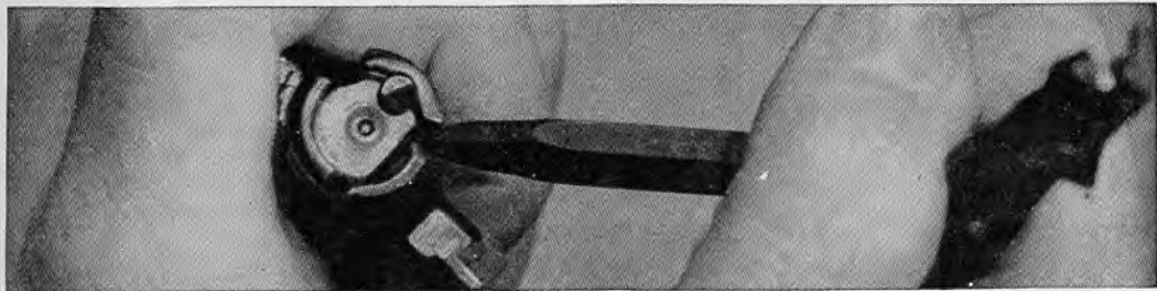
32.9 Pry the extractor out until ejector snaps out against your thumb.
