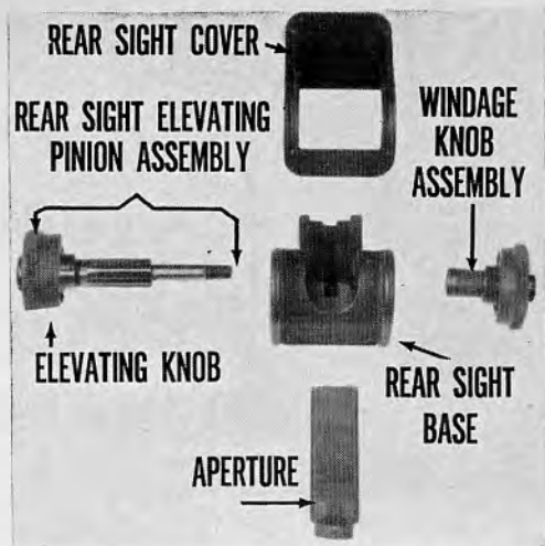
35.17 Parts of rear sight (exploded view).
