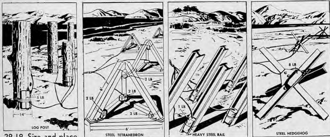
29.19 Size and placement of charges used against common wooden obstacles.
