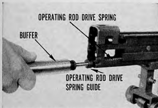
36.5(b) Withdraw the buffer slowly, allowing the operating rod drive spring to expand until the end of the operating rod drive spring guide is exposed at rear of receiver.
