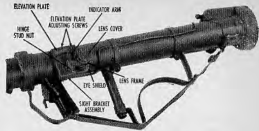
26.3 Reflecting sight of launcher.
