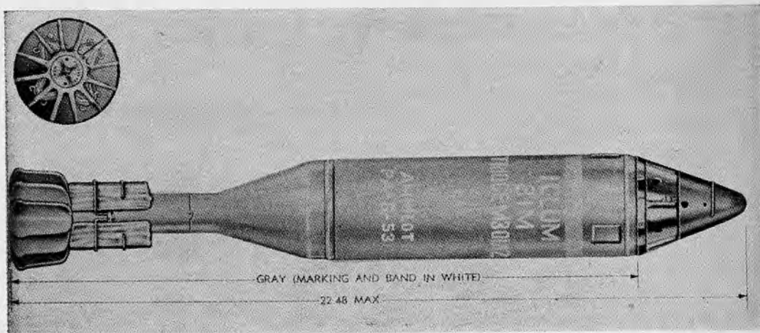
Fig. 30.19(1). Cartridge, 81 millimeter: illuminating, M301A2, w/fuze, time, M84.
