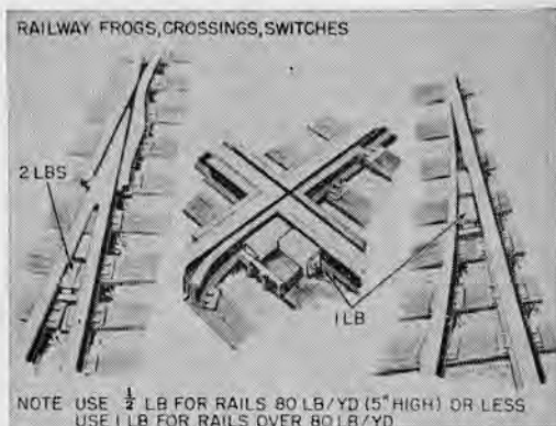
29.21 Placement of charges for demolition of railroad switches, frogs and crossovers.
