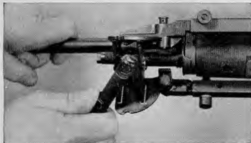
35.42 Loosening the hexagon-shaped nut with the combination tool in preparation for removing the bipod from the rifle.
