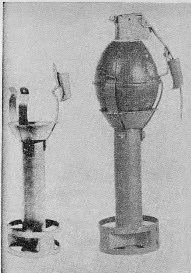
Figure 28.8. M1A2 grenade projection adapter with M26 hand grenade.
