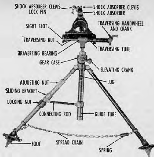
Fig. 30.3 Bipod.
