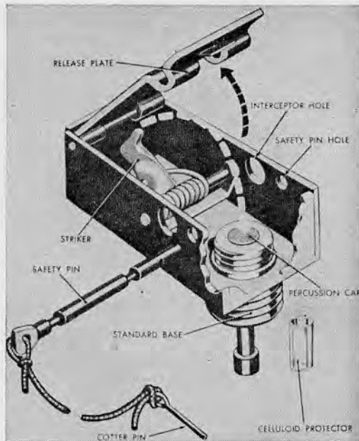
29.33 Pressure-release type firing device, M5,
