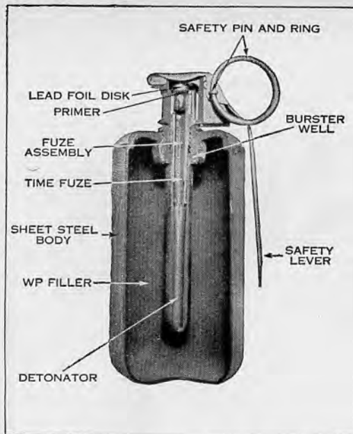
25.5 Smoke Hand Grenade M15.
