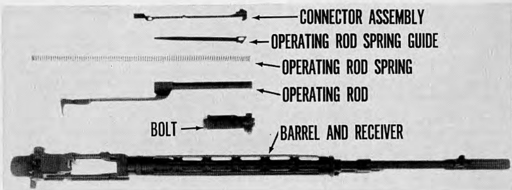
35.8 Parts of barrel and receiver group in the order of disassembly.
