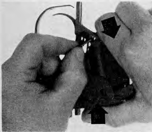
35.21 Replacing the trigger pin.
