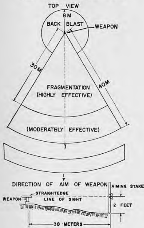
29.26 M18 Casualty Area.
