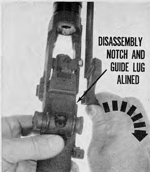
35.7 Removing operating rod.
