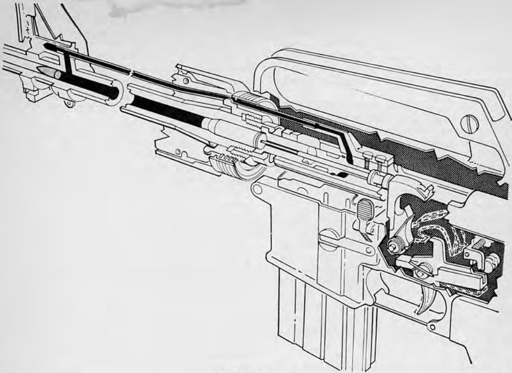
34.26 Firing.
