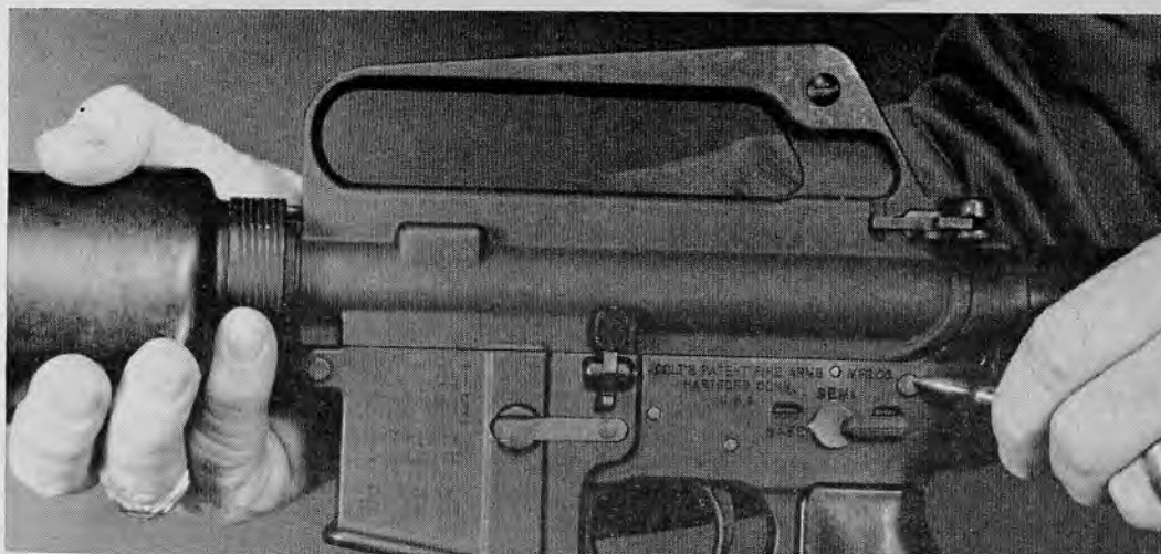
34.2 Pressing the takedown pin to the right with a cartridge.
