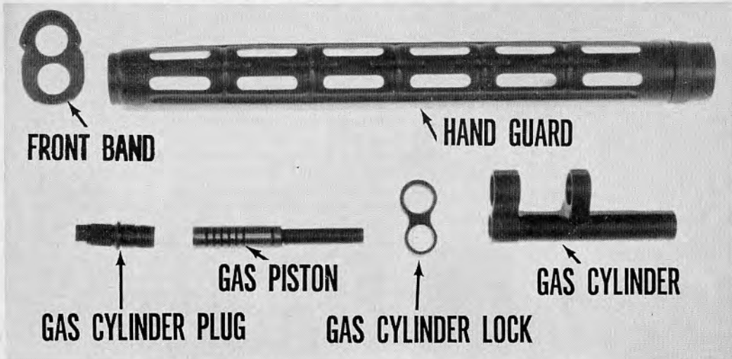
35.12 Parts of the gas system; handguard and front band.
