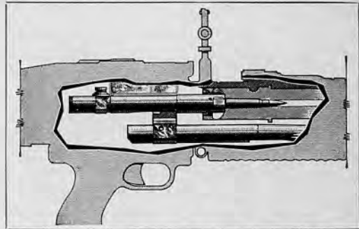
36.27(c) Chambering (cartridge fully seated in chamber).
