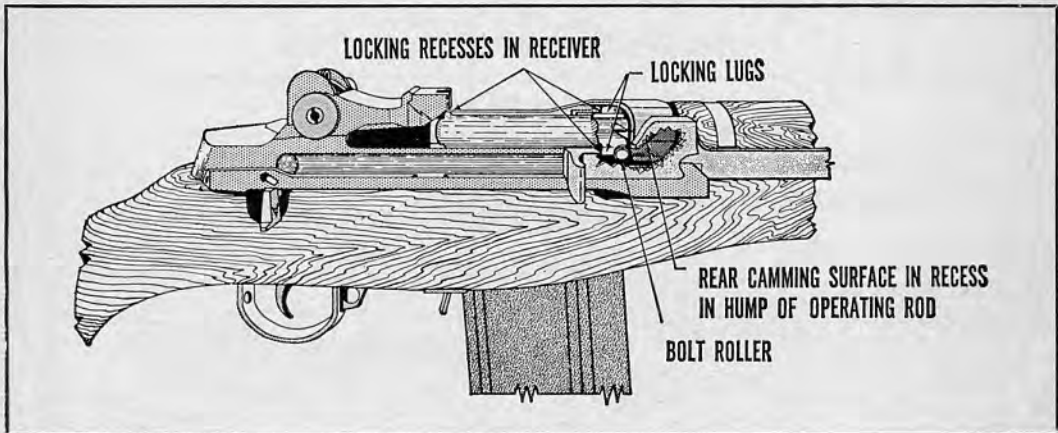
35.25 Locking.
