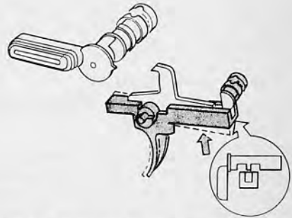
34.35 Showing the selector lever set on AUTO, the center cam blocking the disconnect. Inset shows end view of selector lever in the AUTO position.
