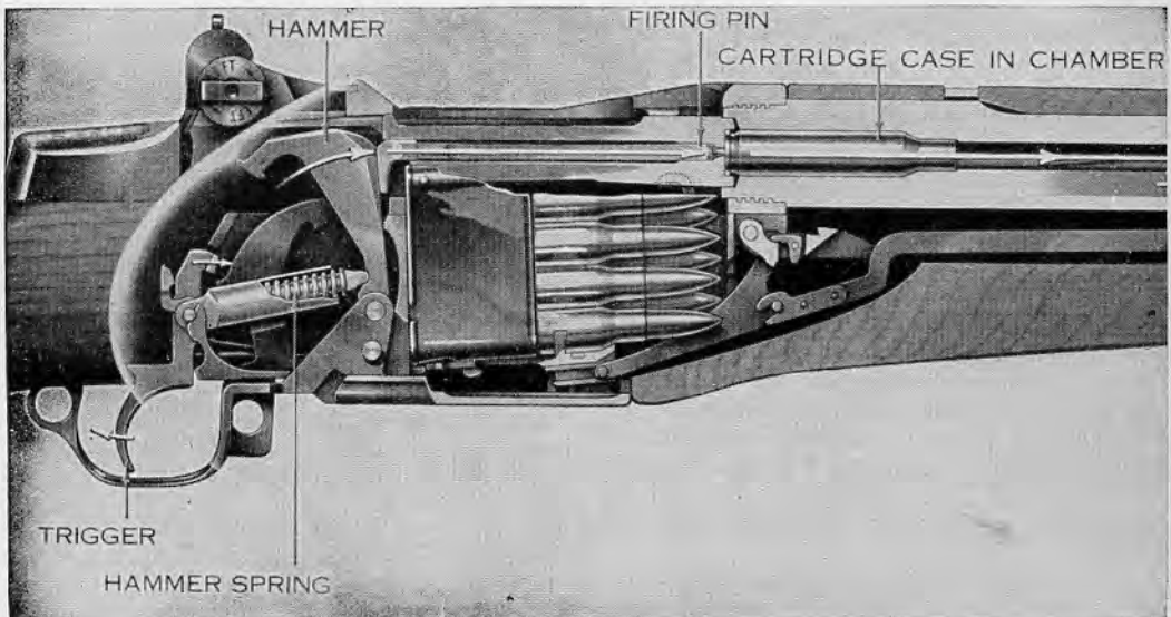
32.10 The hammer strikes firing pin and ignites primer at base of cartridge.
