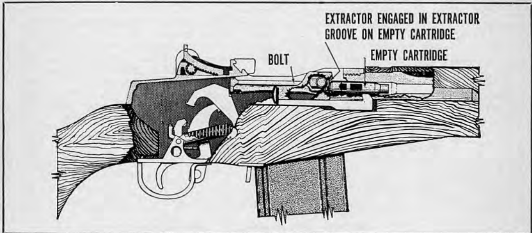
35.29 Extracting.
