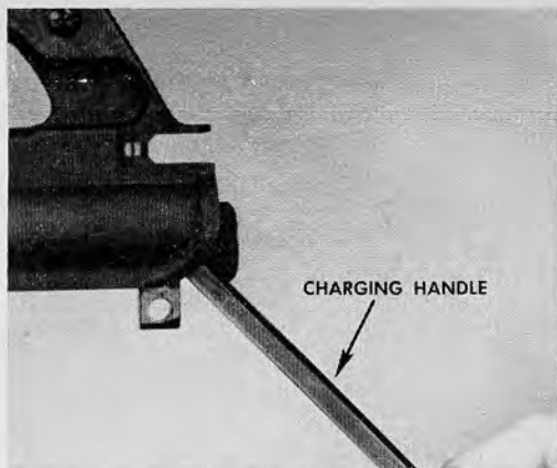
34.8 The charging handle being removed.
