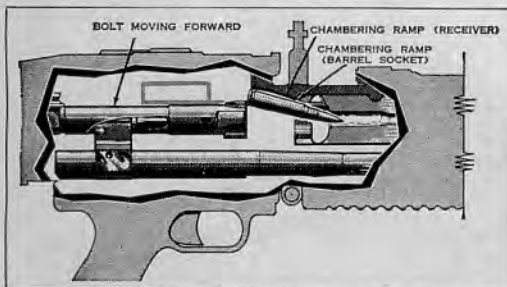
36.27(b) Chambering (cartridge being deflected into chamber).
