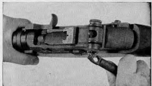
35.34 Combination tool used as offset screwdriver.
