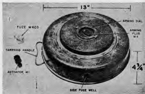
29.30 M15 Anti-tank Mine.
