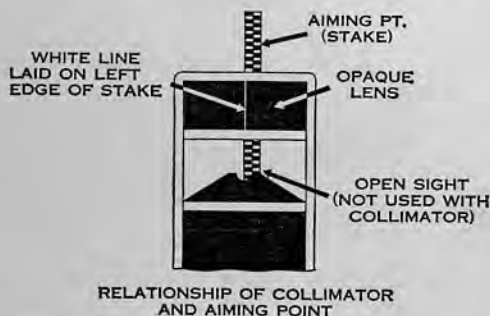
39.5 Collimator, correct sight alignment.
