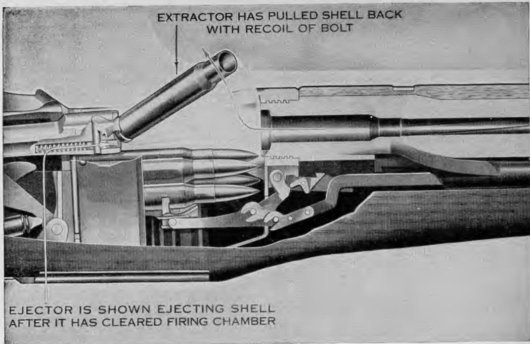
32.12 The ejector throws the empty cartridge out to the right.
