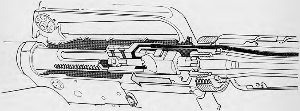
34.29 Extracting.
