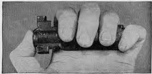
32.8 Hold little finger over firing pin. Hold thumb firmly over extractor.
