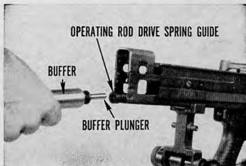
36.5(c) Remove the buffer by pulling the buffer plunger from the operating rod drive spring guide.
