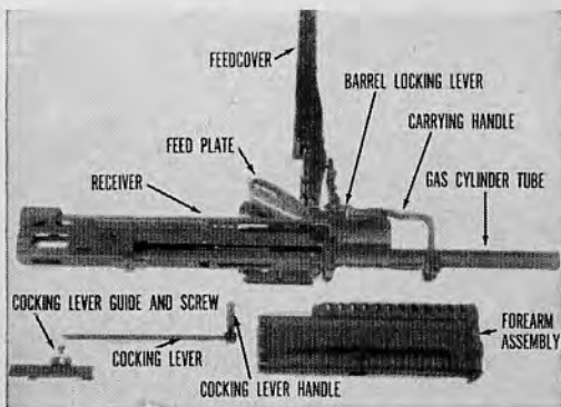
36.20(f) Receiver group disassembled in detail.
