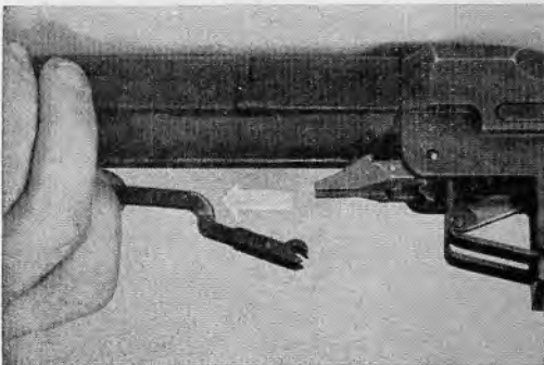
32.5(2) Disengage follower rod from arm by pressure toward muzzle.
