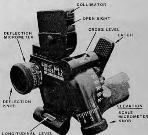
39.4 The M4 Sight.
