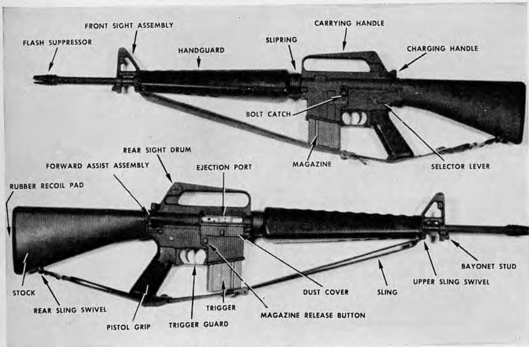
34.1 The Rifle, 5.56-mm. Right and left side views.
