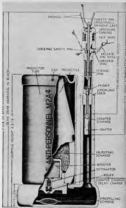
29.24 Anti-personnel Mine M2A4 and combination mine fuze M6A1.
