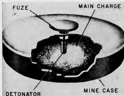
29.22 Components of a typical mine.
