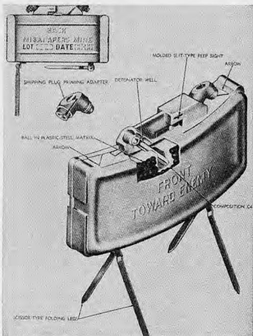
29.27 Anti-personnel Mine M18A1.
