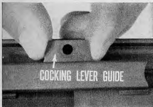
36.20(b) Remove the cocking lever guide by rotating it downward, away from the receiver.
