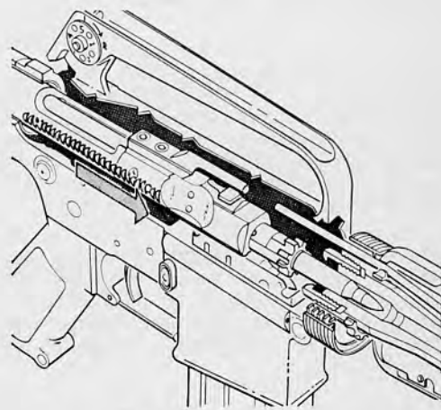
34.33 Chambering.
