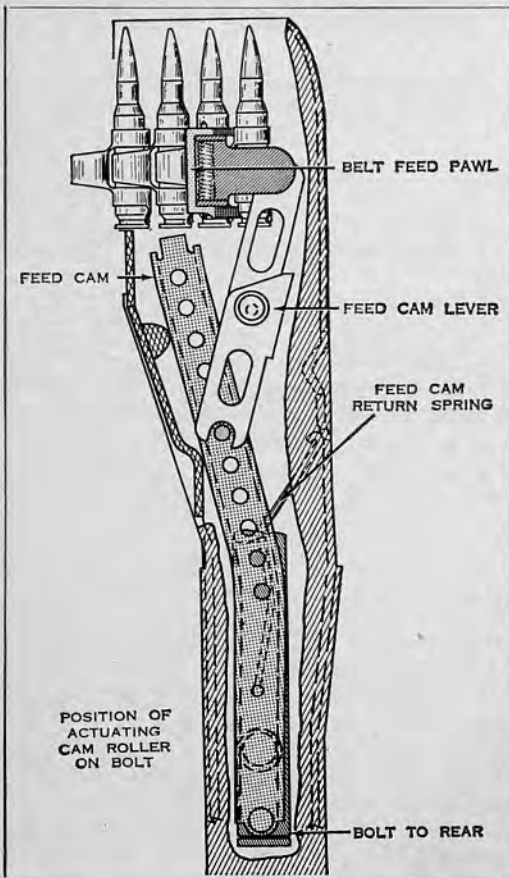
36.26(a) Feeding (bolt to the rear).
