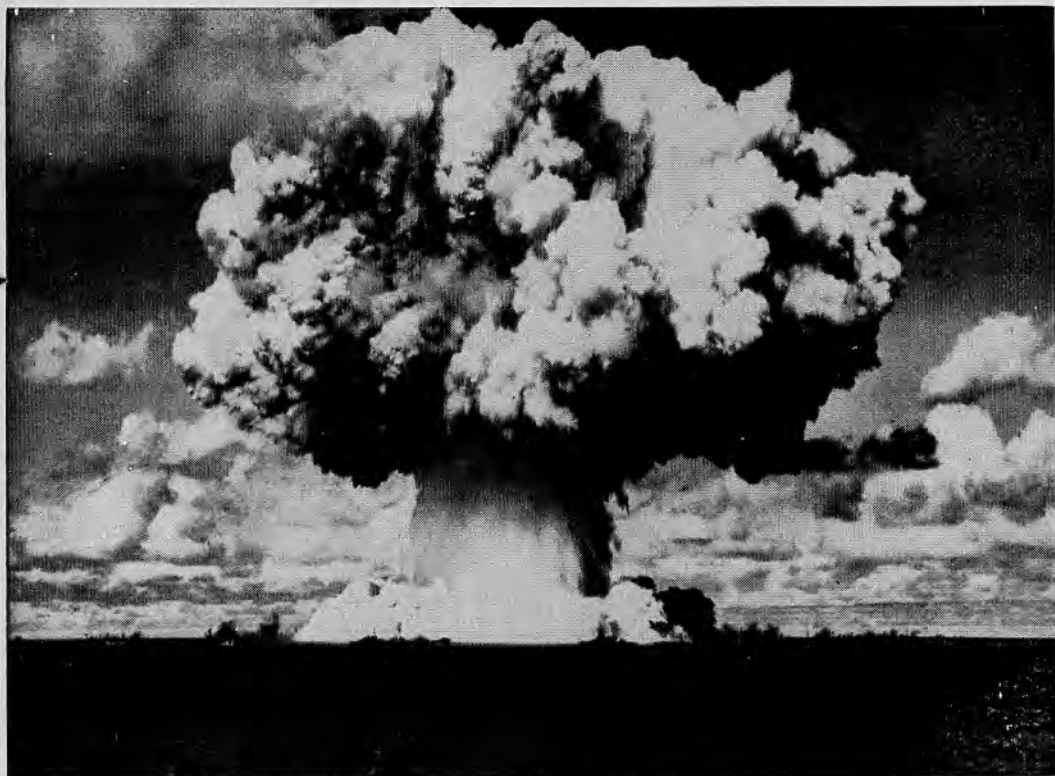
22.1 A typical nuclear burst.
