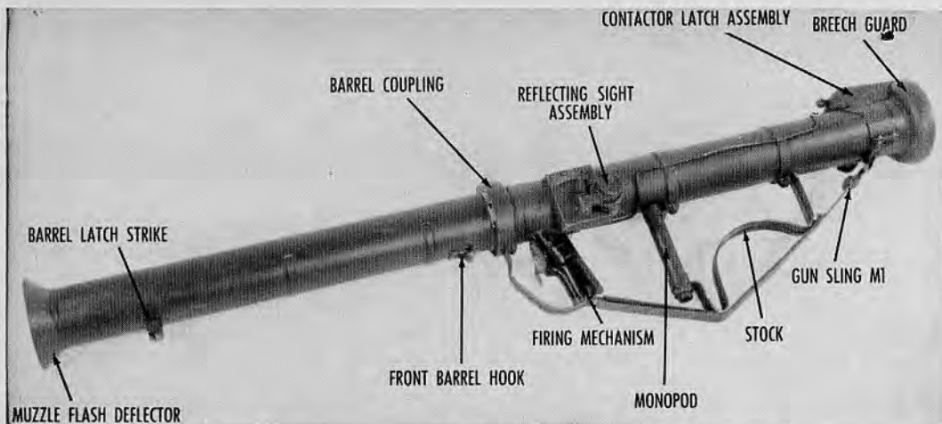
26.1 Nomenclature of the M20 launcher.
