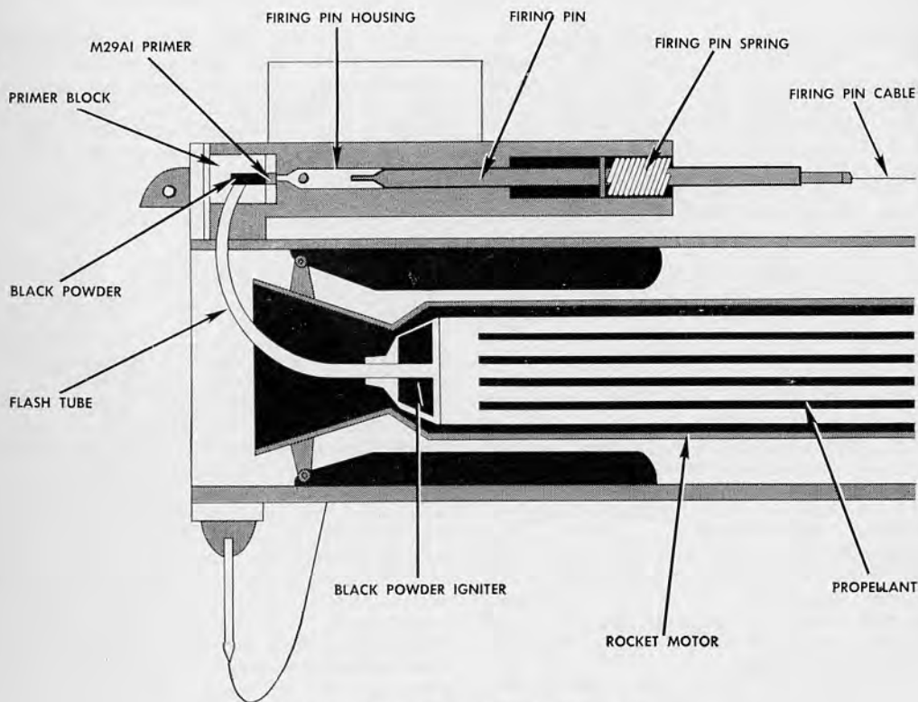
33.13 Rocket motor ignition system.
