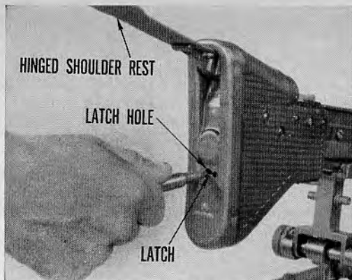
36.4(b) Raise the hinged shoulder rest and insert the nose of a cartridge into the latch hole, thereby depressing the latch.
