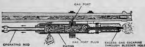
36.30(a) Unlocking (action of the gas).
