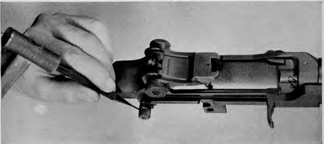
35.37 Removing the selector shaft pin.
