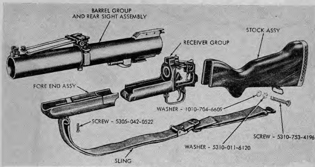
37.3 M79 disassembled into groups.
