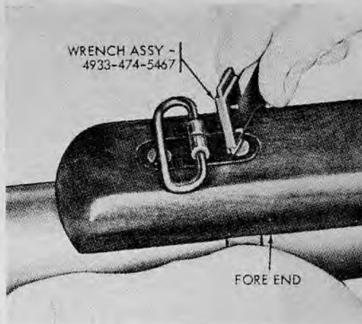
37.5 Removing the fore end screw.
