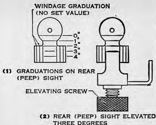
Figure 28.4. Rear peep sight of the M15 sight.
