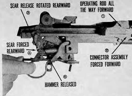
35.39 Effects of forward movement of connector assembly.
