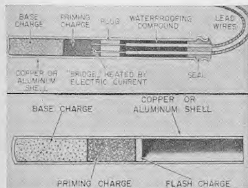
29.3 Electric and non-electric blasting caps.
