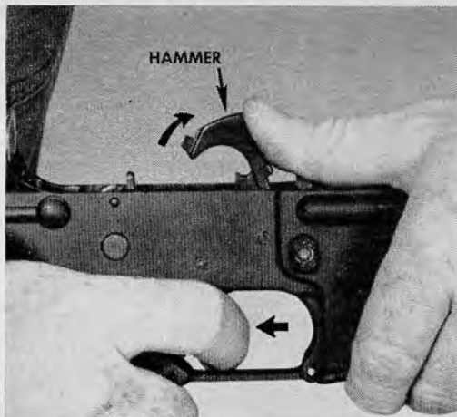
34.15 Lowering the hammer.
