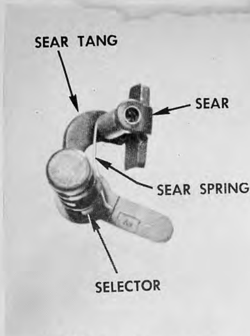
34.24 Position of sear tang and sear spring on the selector lever.
