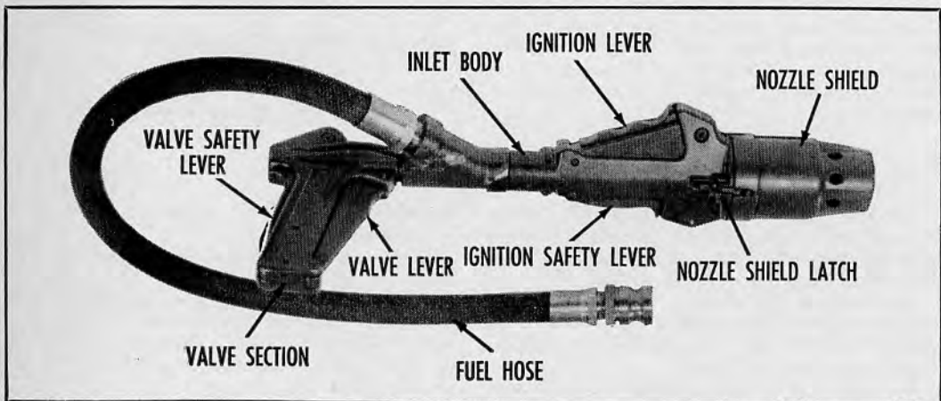
27.4 Gun group nomenclature.
