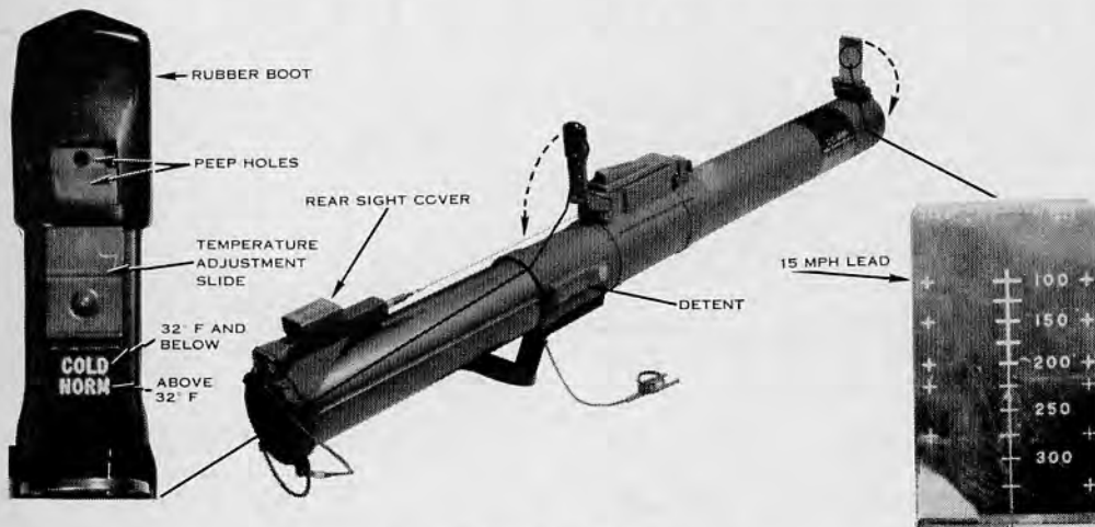
33.8 Front and rear sights.
