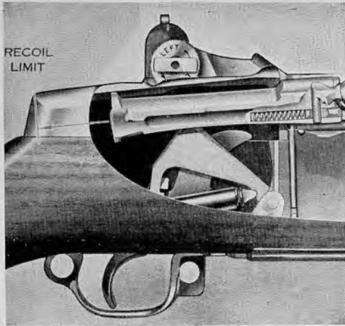
32.13 Bolt rides over hammer, forcing hammer back and thus cocking it.
