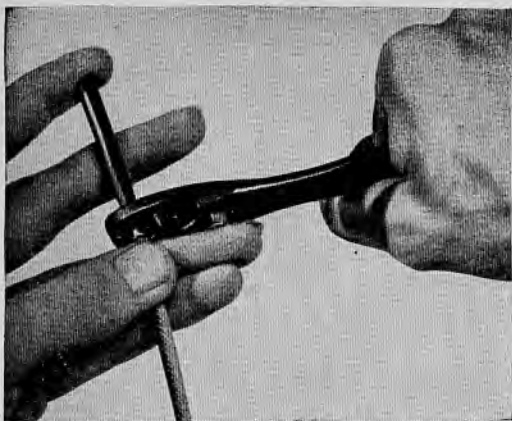
29.7 Method of using Cap Crimpers.
