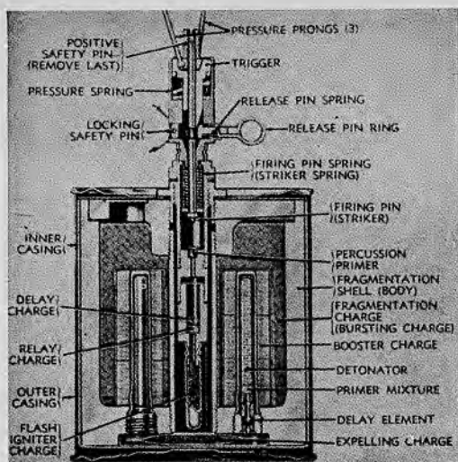
29.25 Anti-personnel Mine M16.
