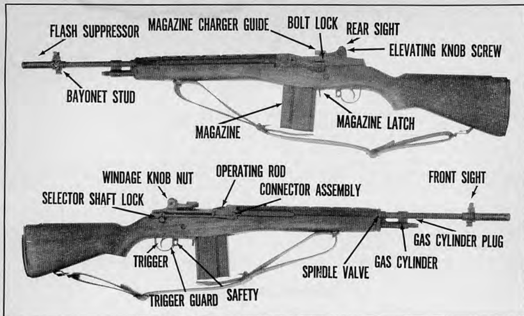
35.1 The M14 Rifle.
