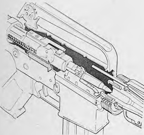
34.32 Feeding.
