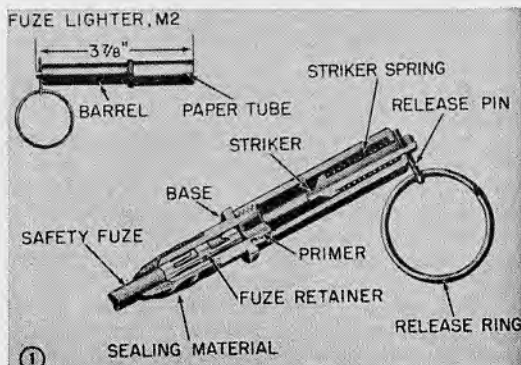
29.6 Weatherproof Fuze Lighter, M2.
