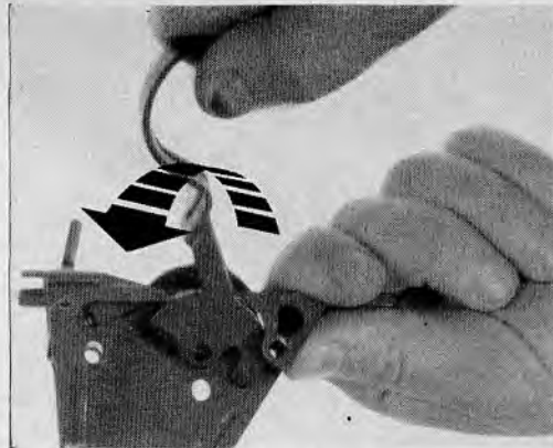
35.10 Removing the trigger guard.
