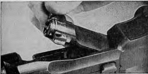
32.7 Lift the bolt up and out to the right front.
