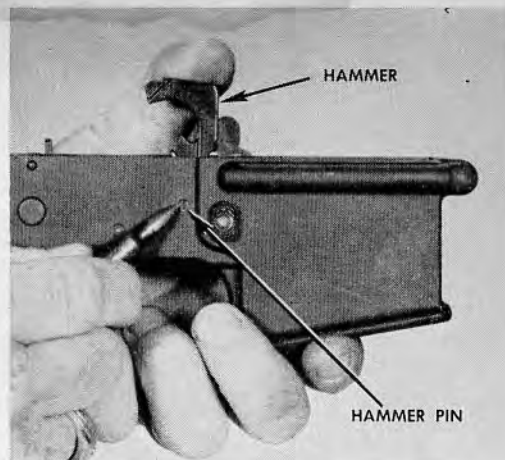
34.16 Pressing out the hammer pin.
