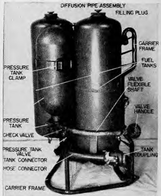
27.2 Tank group nomenclature.
