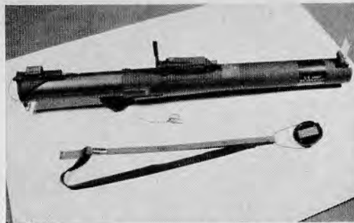
33.2 M72 opened and in firing position.
