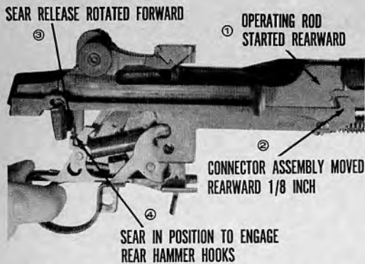
35.38 Effects of rearward movement of connector assembly.
