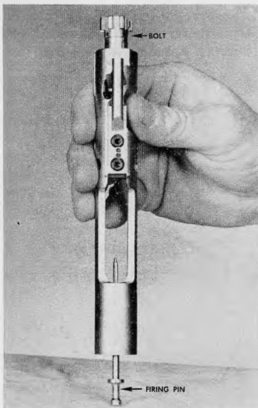
34.10 Removing the firing pin.
