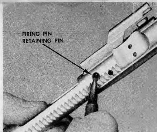
34.9 Pressing out firing pin retaining pin.
