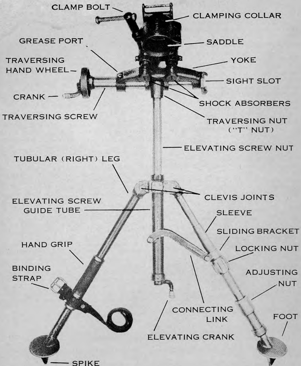
39.6 Mount, Bipod, M5.
