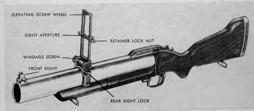
37.2 Grenade launcher M79, left front view.
