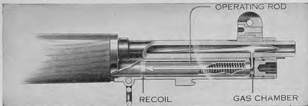
32.11 Gas strikes piston and drives operating rod to the rear.
