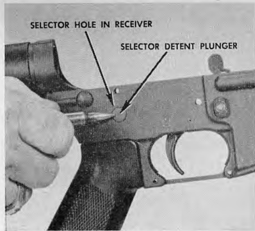
34.20 Removing the selector lever.
