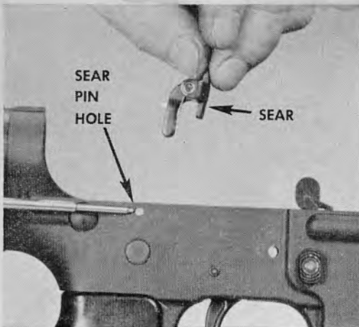
34.19 Removing the automatic sear.
