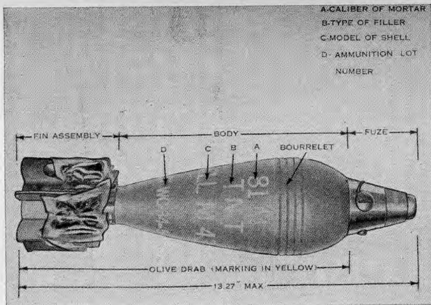
Fig. 30.18 HE Shell, M43A1, with PDF, M52.
