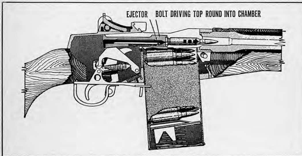
35.24 Chambering.
