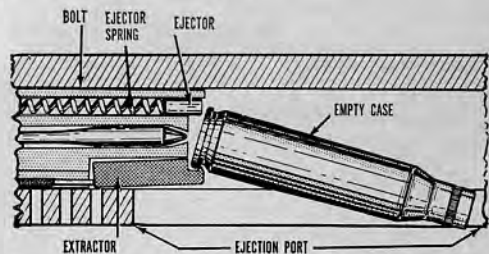
36.31 Extraction and ejection.
