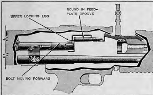
36.27(a) Chambering (upper locking lug of bolt stripping round from the belt).
