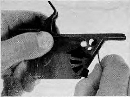
35.20 Replacing the safety spring.
