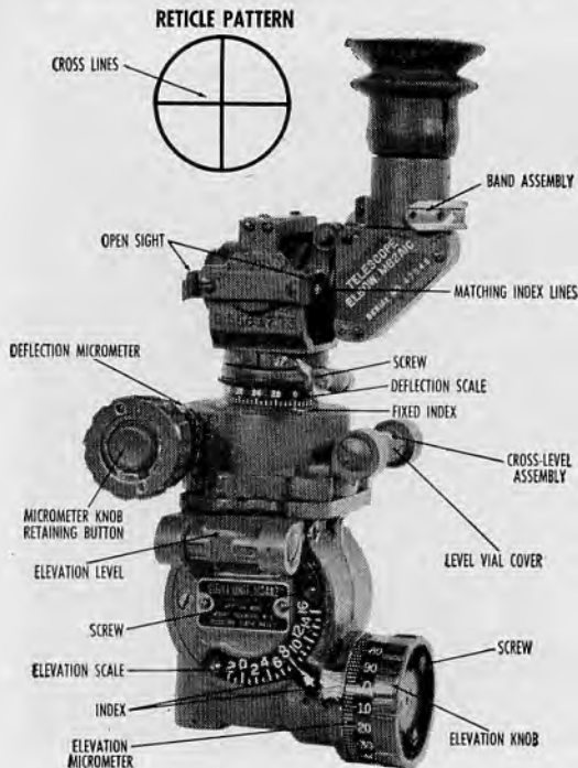
Fig. 30.9(1) Sight unit, M34A2.
