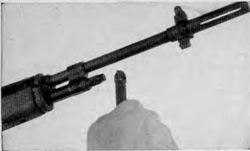
35.35 Combination tool used as wrench.
