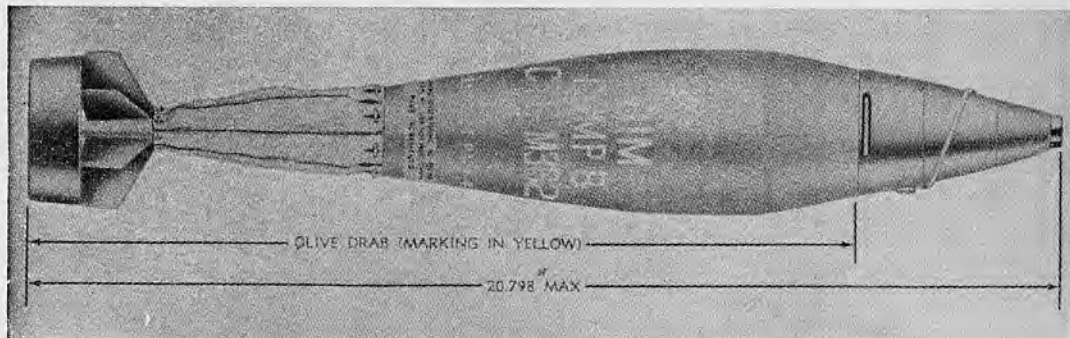
Fig. 30.17 Cartridge, 81 millimeter: HE, M362, w/fuze, PD.
