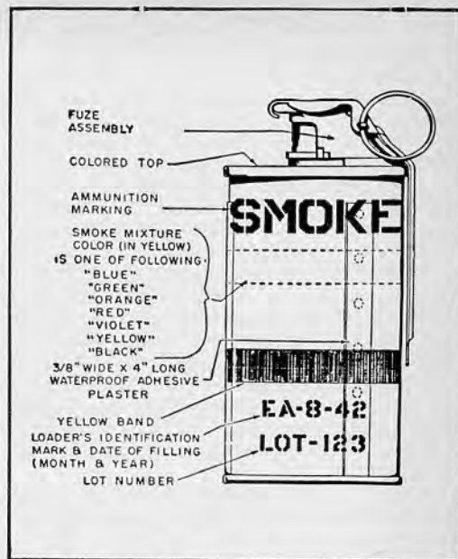
25.6 Colored Smoke Hand Grenade M18.
