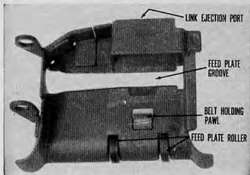
36.25 Important parts of the feedplate.
