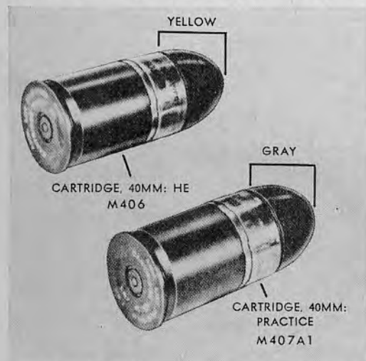
37.8 Cartridges used with the M79.
