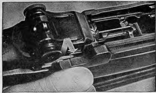
32.6(2) Then with an upward and outward movement disengage operating rod handle from bolt operating lug and receiver.
