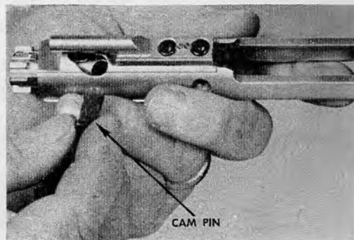
34.11 Removing the cam pin.
