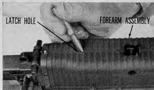
36.20(d) Turn the receiver group so that the cover is down. Insert the nose of a cartridge in the latch hole at the bottom rear of the forearm assembly.
