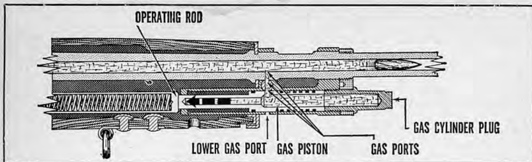
35.27 Action of the gas.
