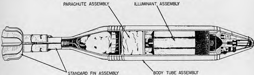
Fig. 30.19(3). Cut away view.
