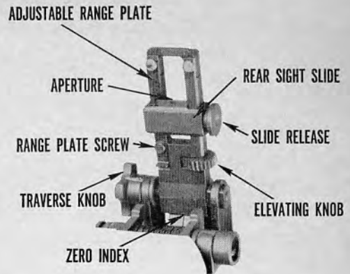
36.2 Rear Sight.
