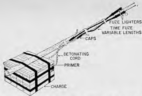
29.16 A pole charge primed with detonating cord.
