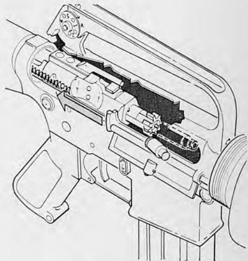
34.30 Ejecting.
