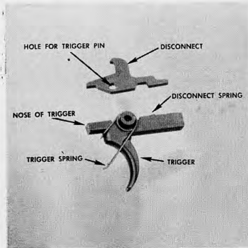
34.22 Trigger and disconnect separated.
