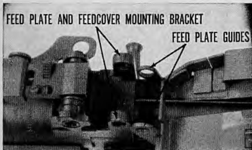
36.24 Raise the feedplate from the receiver and remove it.
