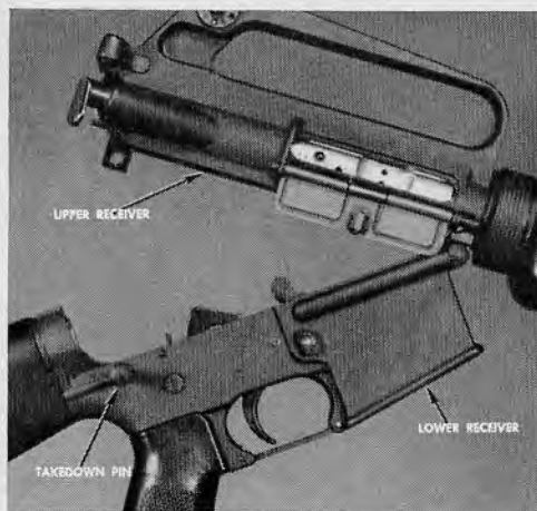
34.3 Upper receiver swings free of the lower receiver.
