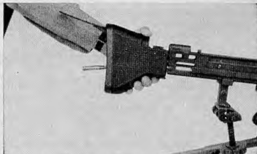
36.4(c) Leaving the cartridge depressing the latch, remove the butt stock group by pulling to the rear.
