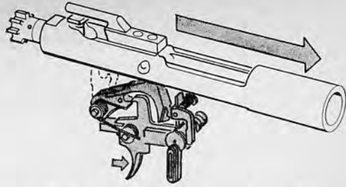
34.31A Cocking (showing hammer caught by nose of the trigger).
