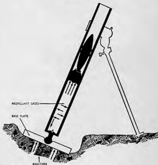
Fig. 30.7 Functioning of smoothbore mortar.
