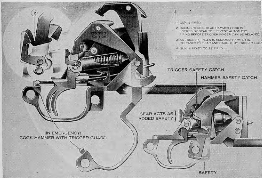
32.15 Trigger and safety functioning.
