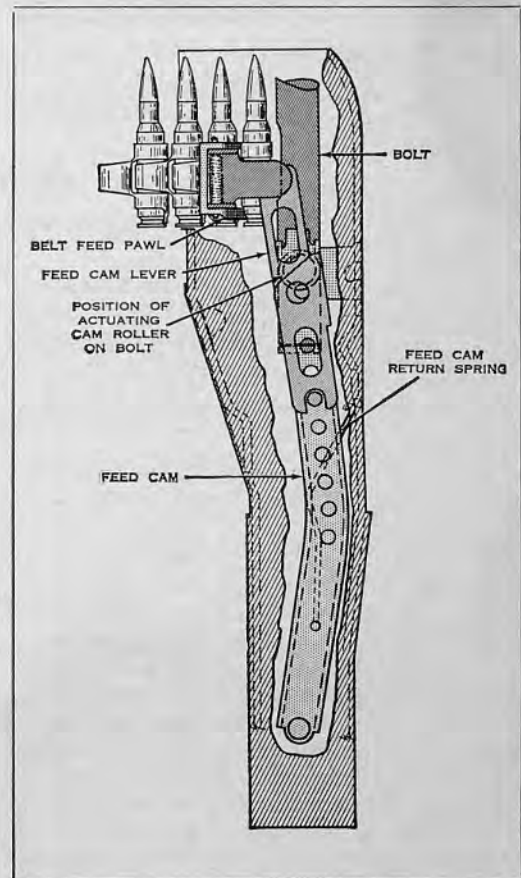
36.26(b) Feeding (bolt forward).
