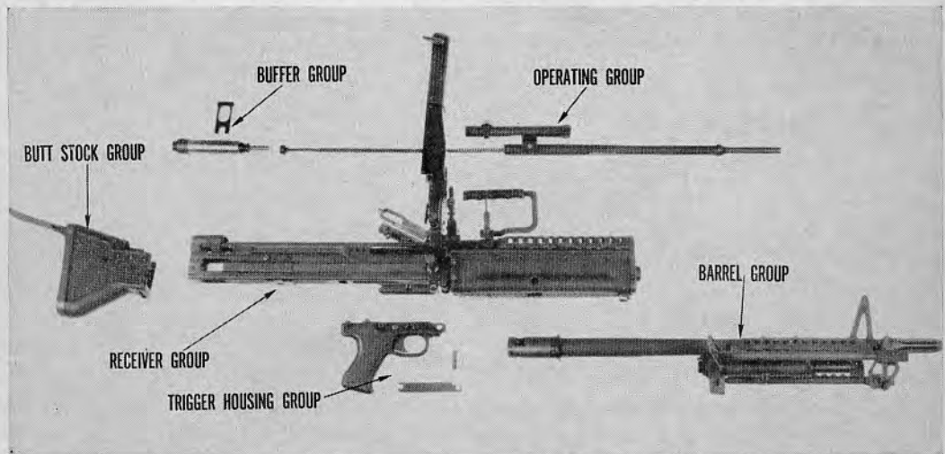
36.3 Six major groups disassembled.
