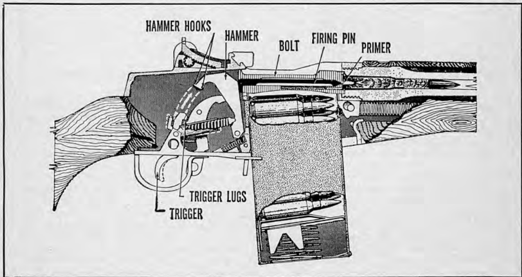
35.26 Firing.
