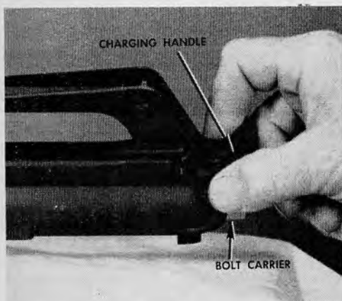
34.6 Pulling the charging handle to the rear.
