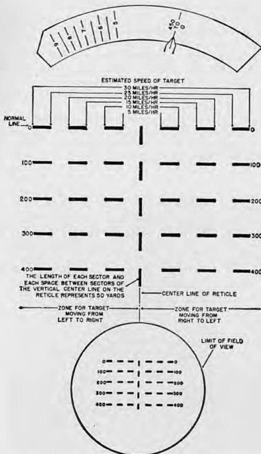
26.4 Ladder type reticle pattern and elevation plate used with it.
