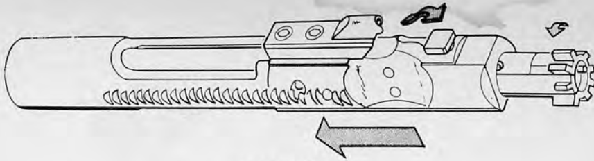
34.28 Unlocking.
