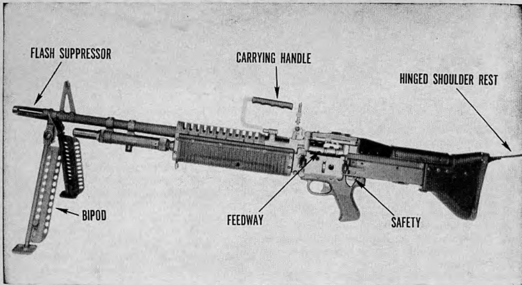
36.1(1) Machine Gun, 7.62-mm., M60, Bipod mounted.
