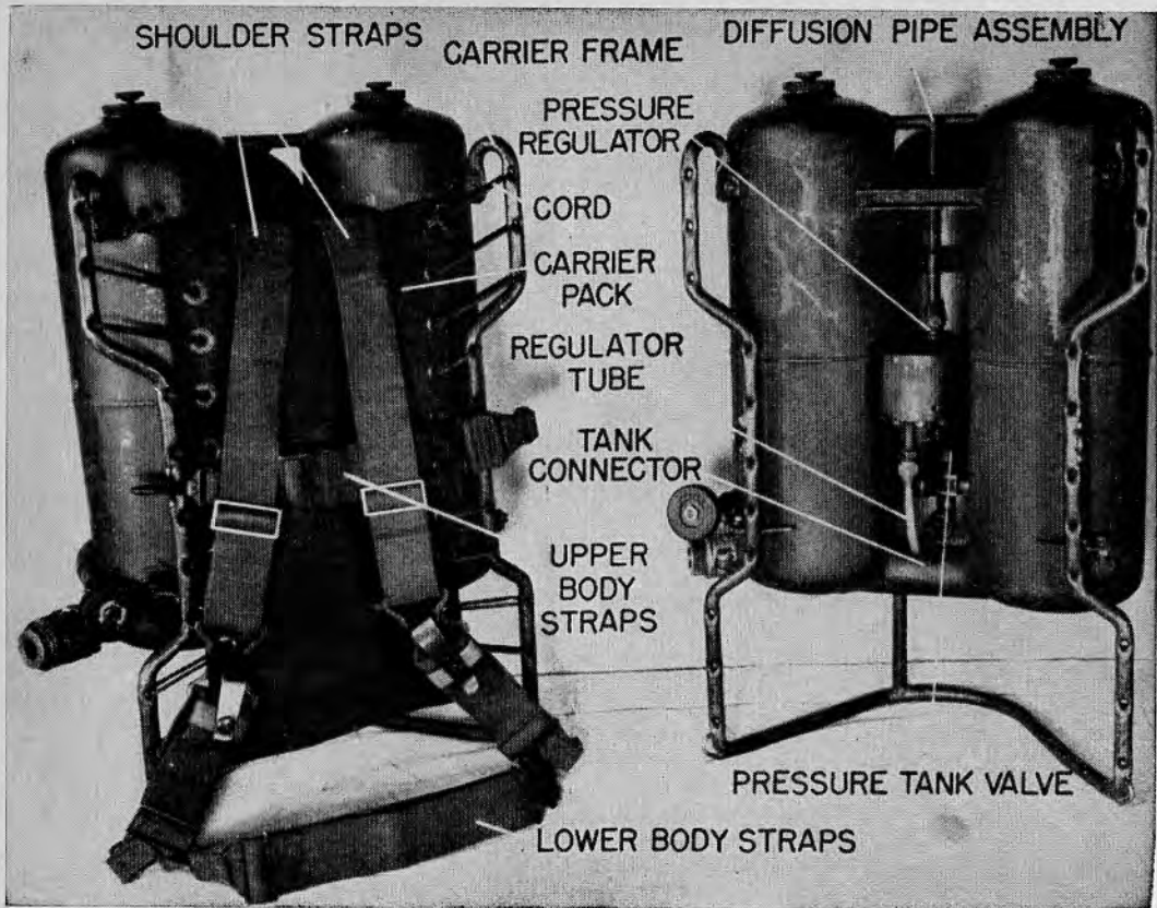
27.3 Rear view of tank group.
