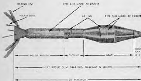
33.3 66-mm. High Explosive Antitank Rocket.
