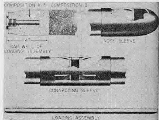
29.13 Components of an M1A1 bangalore torpedo.
