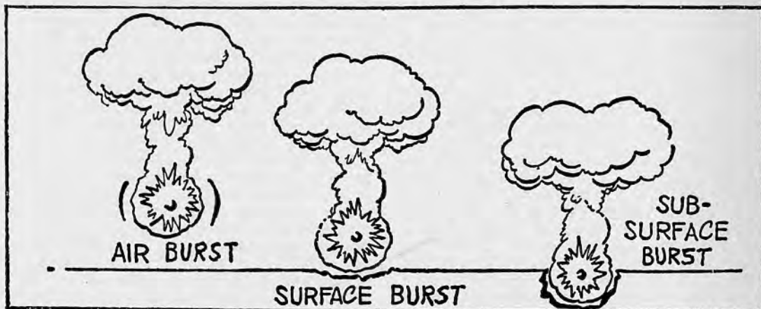
22.3 The three types of nuclear explosions.
