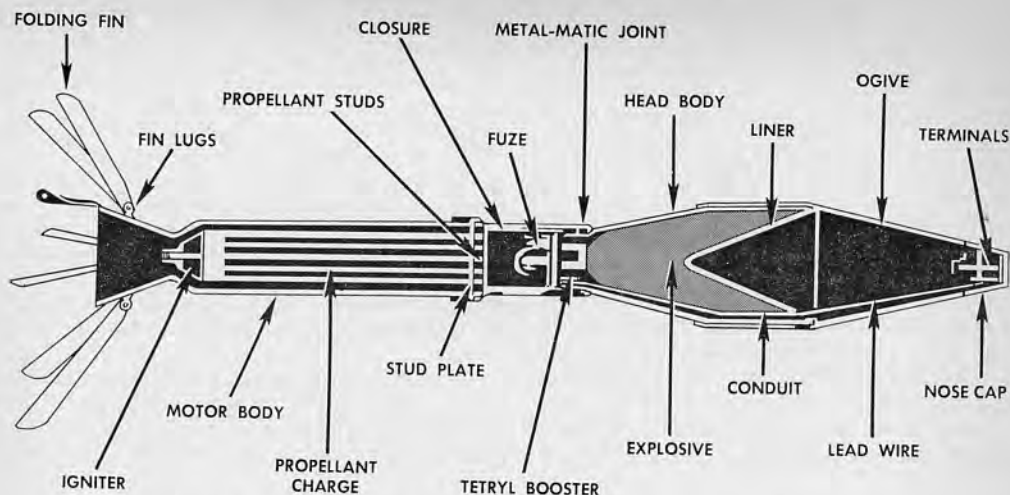
33.12 Cross-section and nomenclature of the 66-mm. HEAT rocket.
