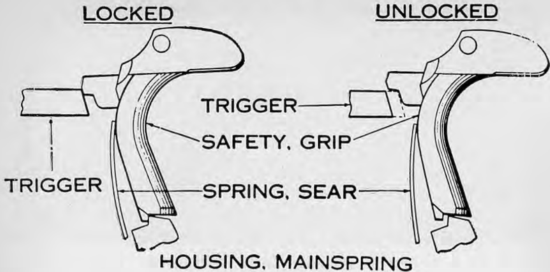
24.7 Grip Safety Mechanism.
