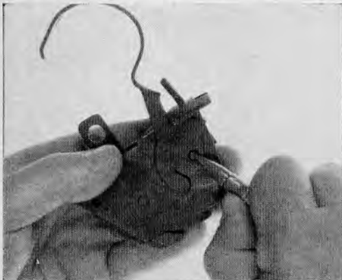
35.9(3) Removing the hammer pin.
