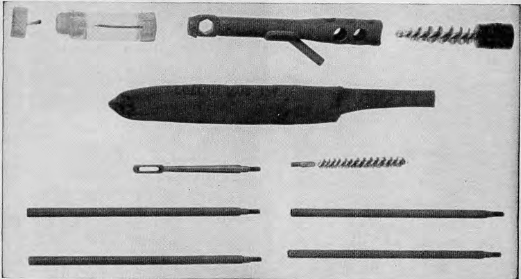
35.32 Cleaning equipment.
