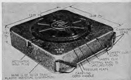
29.31 M19 Anti-tank Mine.
