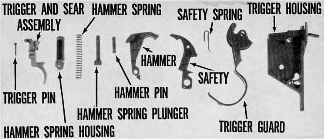
35.11 Parts of firing mechanism assembly in the order of disassembly.
